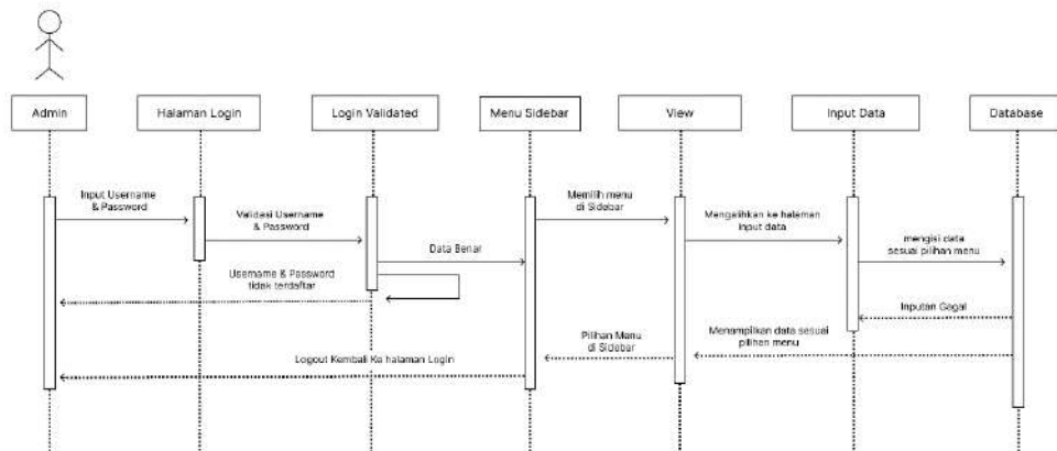
Gambar IV. 5 Sequence Diagram (Admin)
