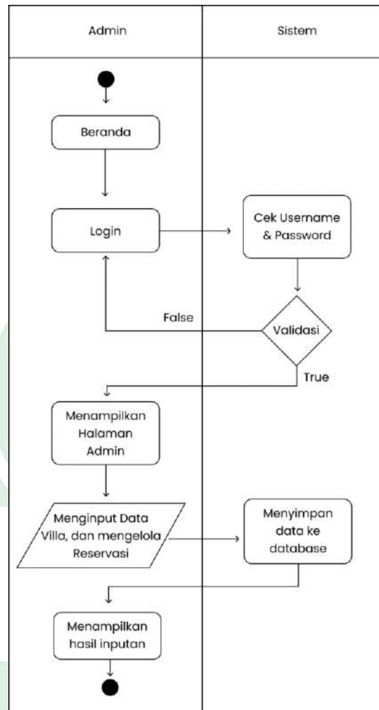
Gambar IV. 8 Activity Diagram Admin
