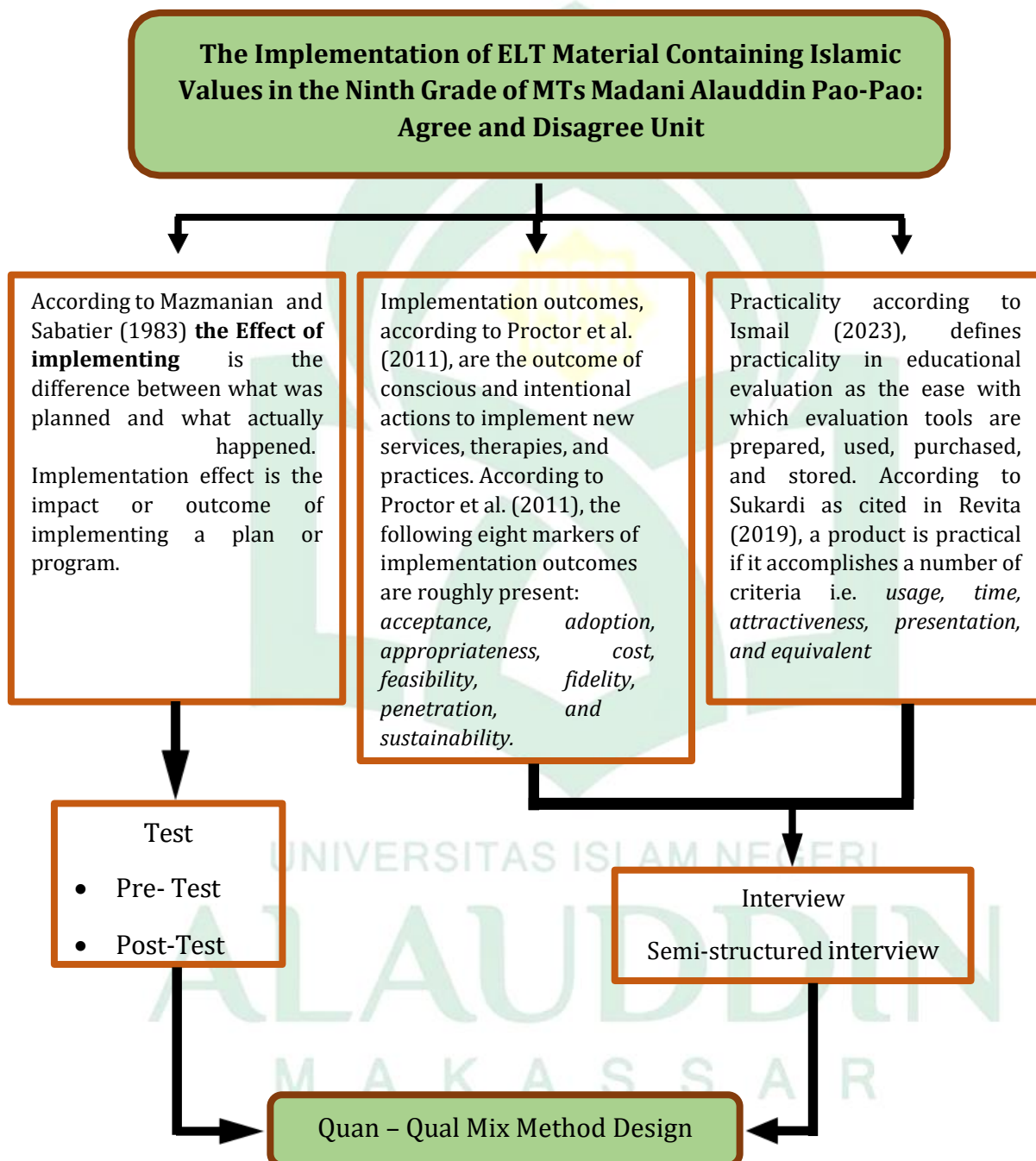
Figure 2. 1 Conceptual Framework
