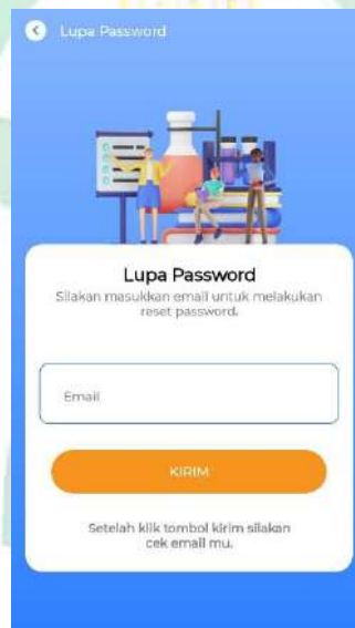
Gambar 2.3 Lupa Password
