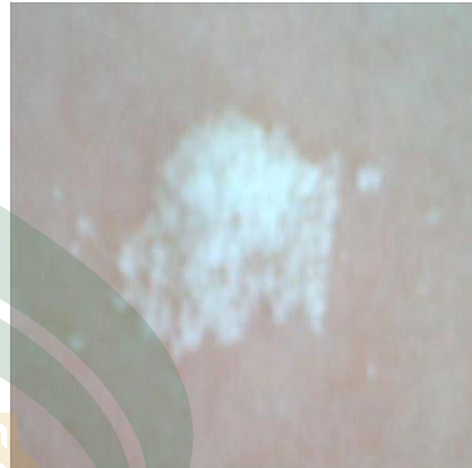
Gambar 8. Asam Tartrat
