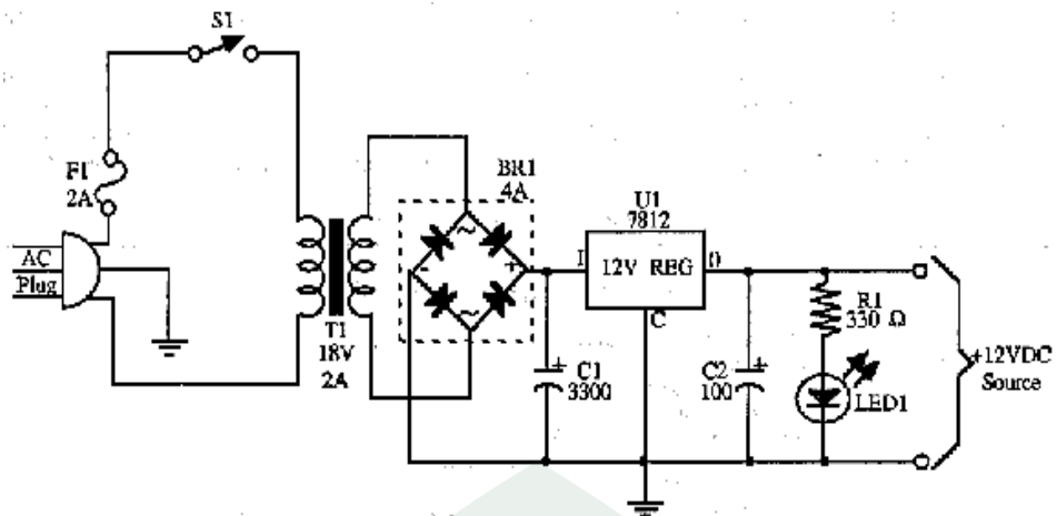
Gambar IV- 5. Rangkaian Power Supply
