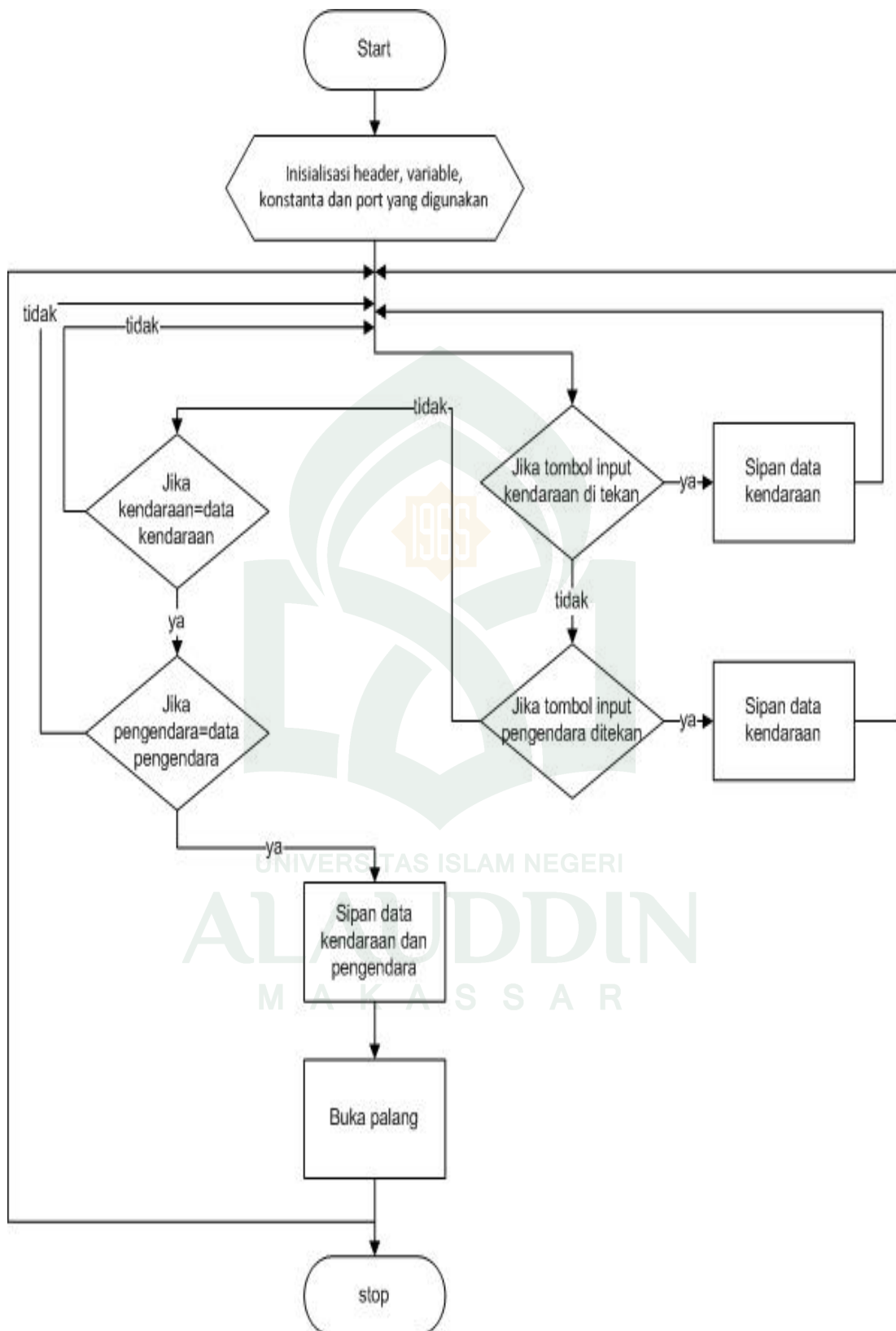
Gambar IV- 11. Flowchart Sistem Parkir
