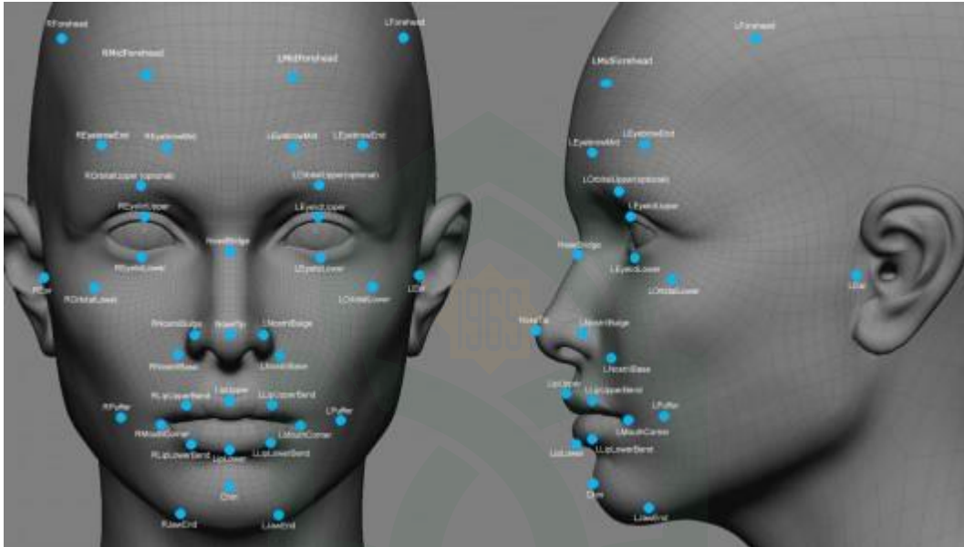
Gambar II- 6. Biometrik wajah
