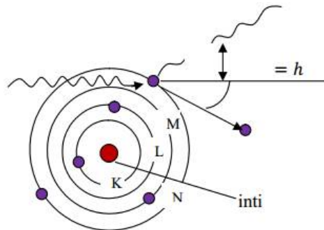
Gambar 2.3 Proses hamburan Compton (Sumber: Gusmavita, 2011)
