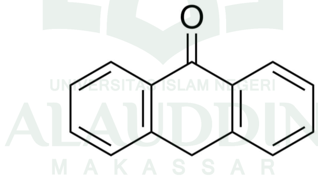
Gambar 1. Rumus struktur Anthrone (9,10-dihydro-9-oxanthracene) (Anton, 2002).
