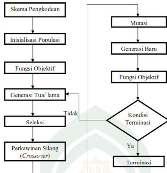
Gambar II.2 Diagram Alir Algoritma Genetika
