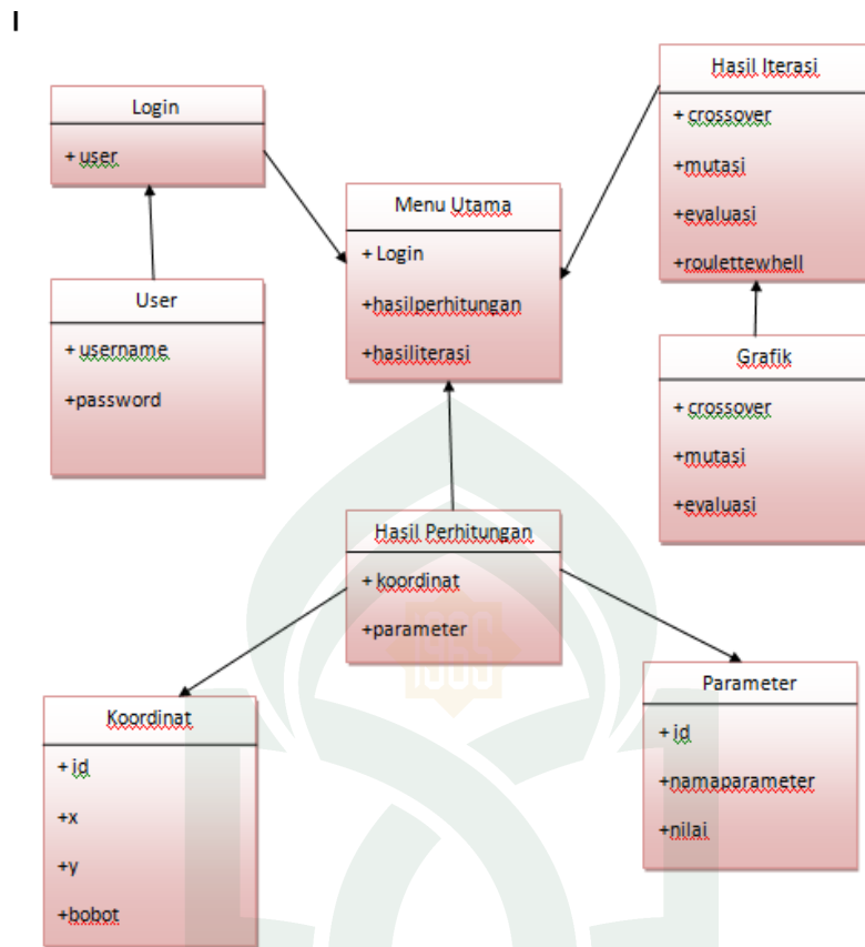
Gambar IV.5. Class Diagram
