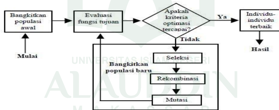
Gambar II.1 Diagram sederhana algoritma genetika ( Kusumadewi, 2003 )
