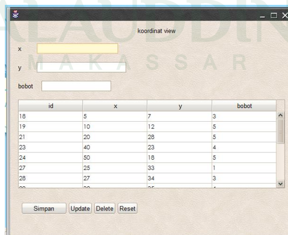
Gambar V. 5. Interface Koordinat
