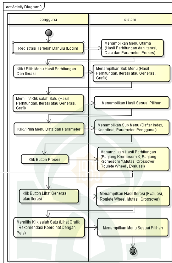
Gambar IV.4. Activity Diagram
