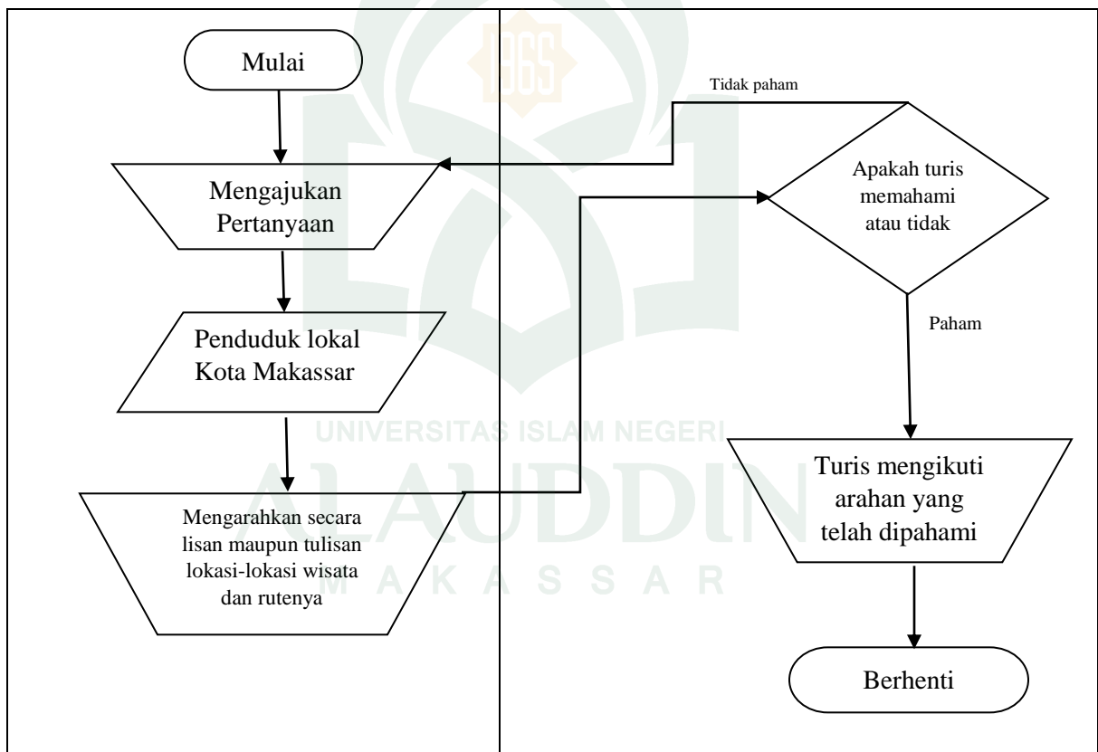
Gambar IV.1 Diagram Flowmap
