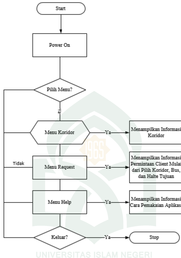
Gambar IV. 14. Flowchart.
