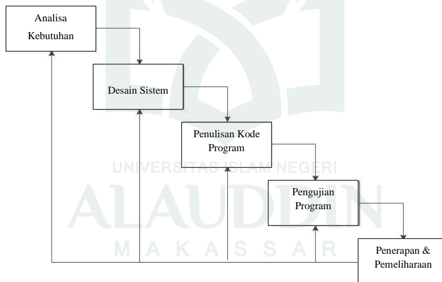
Gambar III.1 Metode Waterfall
