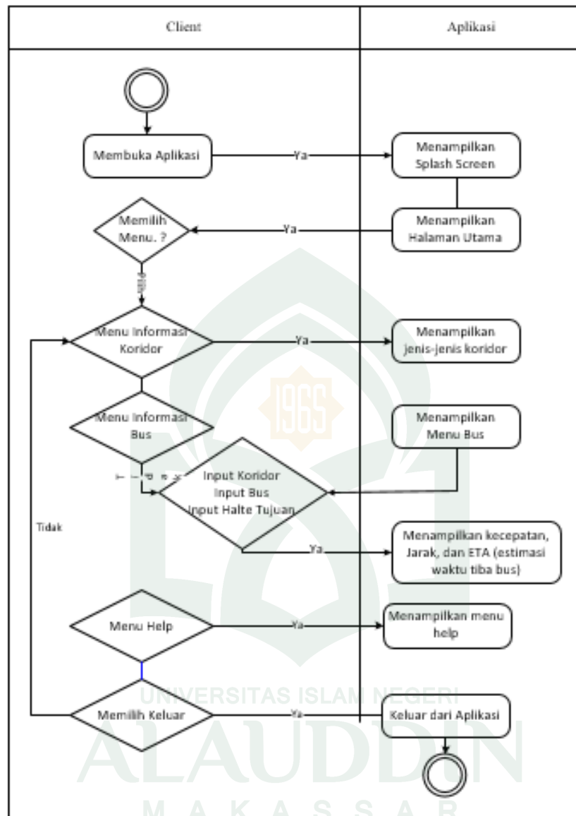
Gambar IV.12. Activity Diagram.
