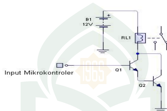
Gambar IV.3 Rangkaian Relay (Aldrin,2017)
