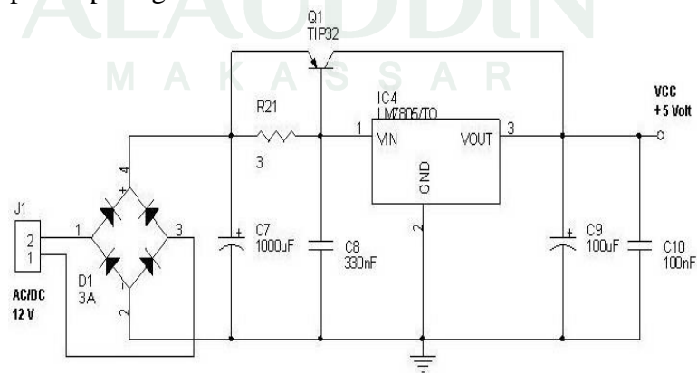
Gambar IV.2 Rangkaian Power Supply (Suhartono, 2017)
