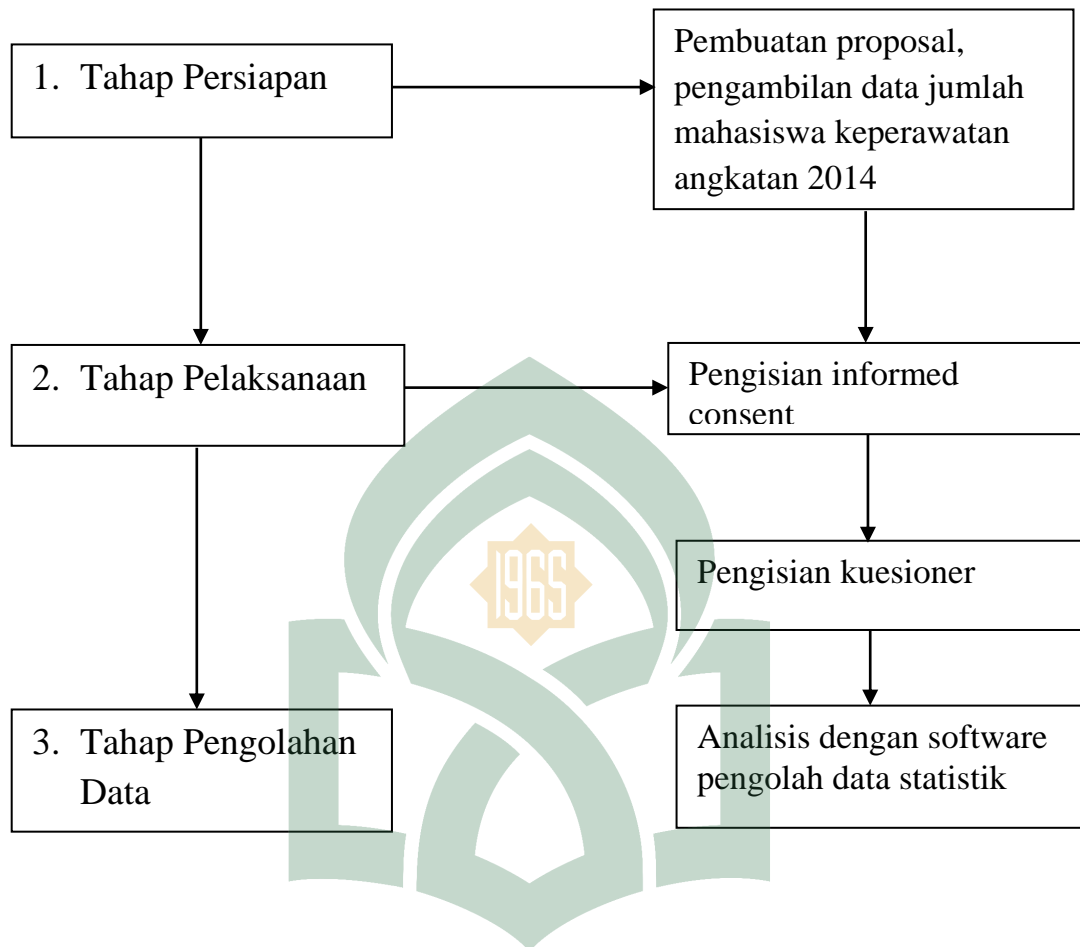
Gambar 2.4 Alur Penelitian
