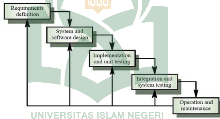
Gambar III.1. Waterfall Model I (Pressman, 2010).
