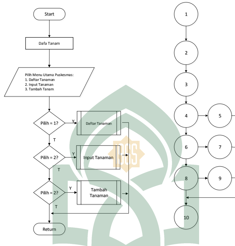
Gambar V.24 Flowchart dan Flowgraph Menu Tanaman.
