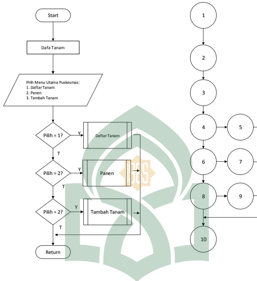
Gambar V.20 Flowchart dan Flowgraph Menu Tanam.
