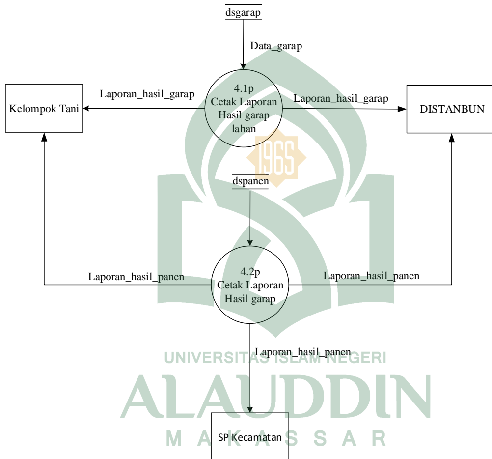
Gambar IV.6 Data Flow Diagram Level 2 proses 4
