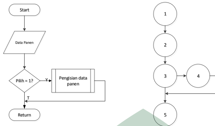
Gambar V.21 Flowchart dan Flowgraph Menu Data Panen
