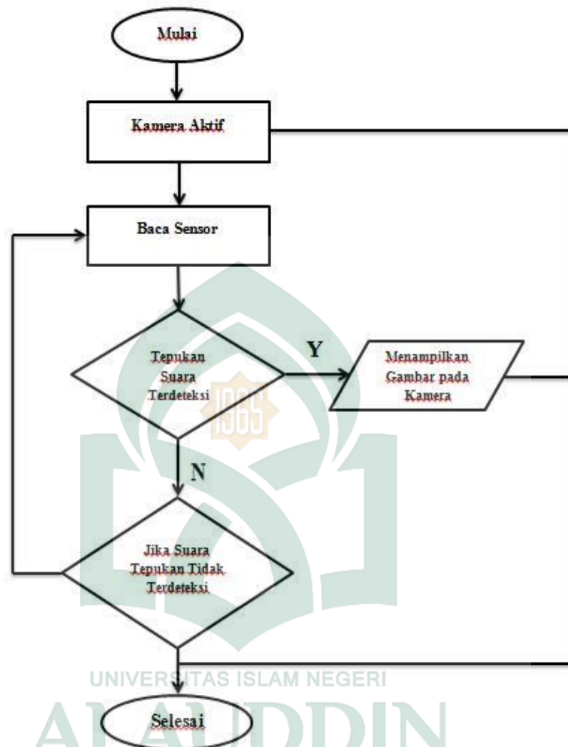
Gambar IV.8. Flowchart (Alur sistem)
