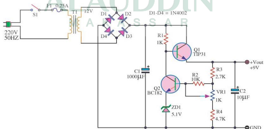
Gambar IV.3. Rangkaian Power Supply
