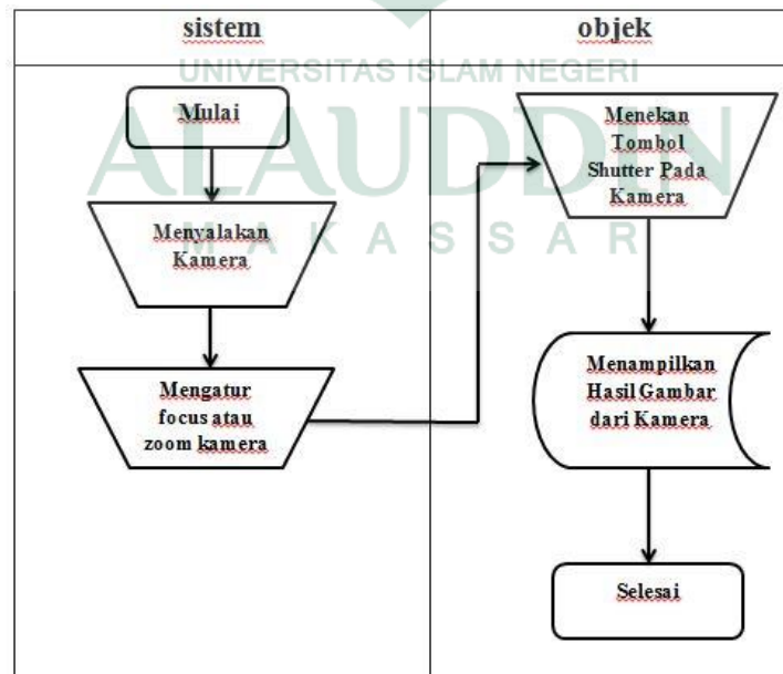
Gambar IV. 1. Flowmap Diagram
