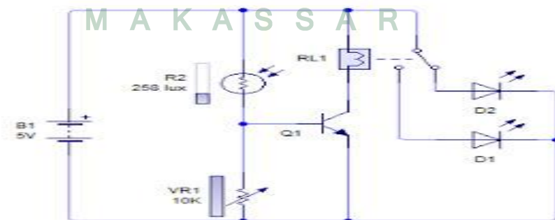
Gambar IV 9. Rangkaian LDR (Chandra, 2015).
