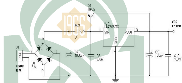
Gambar IV 6 Rangkaian Power Supply (Suhartono, 2015)
