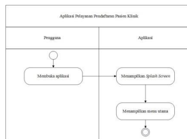
Gambar IV- 5. Activity Diagram Halaman Utama
