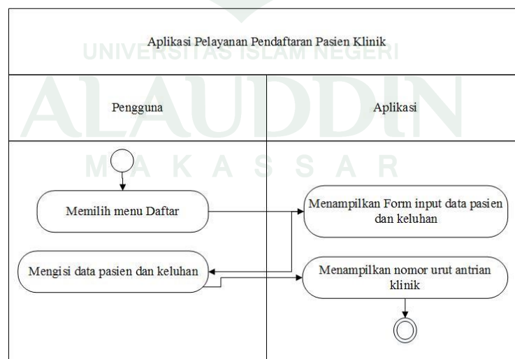
Gambar IV- 7. Activity Diagram Menu Deskripsi Klinik
