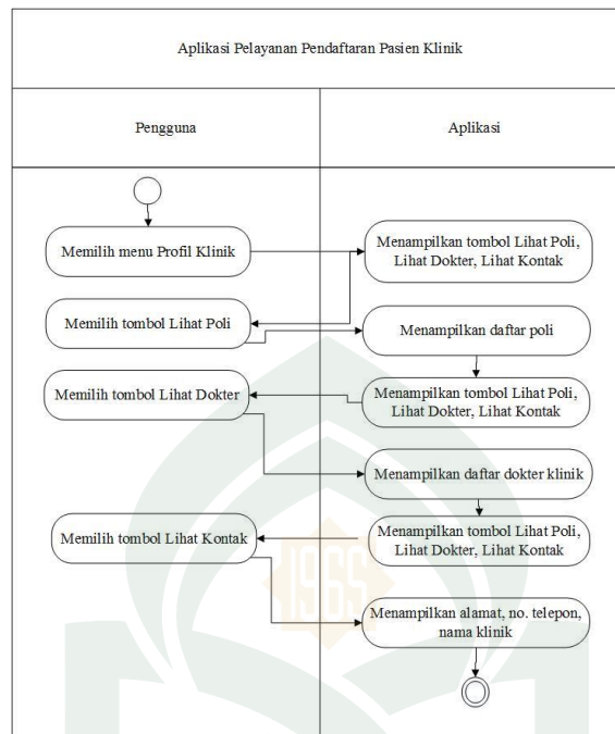
Gambar IV- 6. Activity Diagram Menu Deskripsi Klinik
