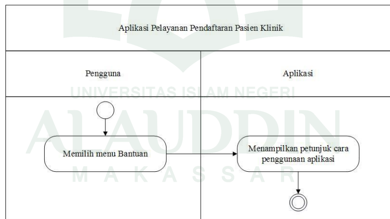
Gambar IV- 9. Activity Diagram Menu Bantuan
