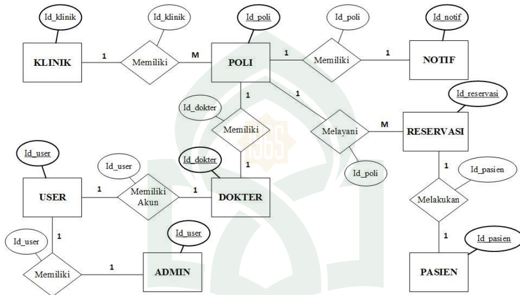
Gambar IV- 19.ERD (Entity Relational Diagram)
