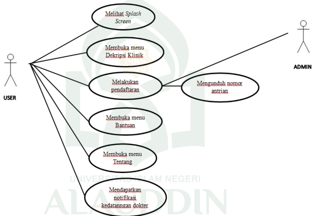
Gambar IV- 3. Use Case Diagram
