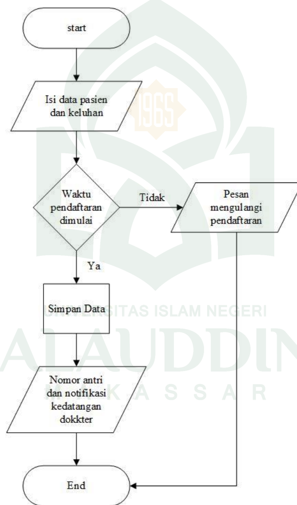
Gambar IV- 12. Flowchart (Alur Program)
