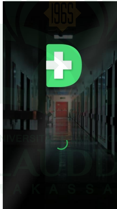
Gambar V- 1. Antarmuka SplashScreen
