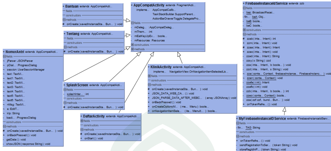
Gambar IV- 4. Class Diagram
