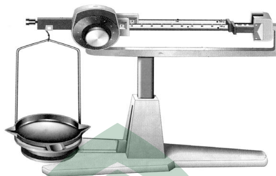
Gambar 6: Neraca
