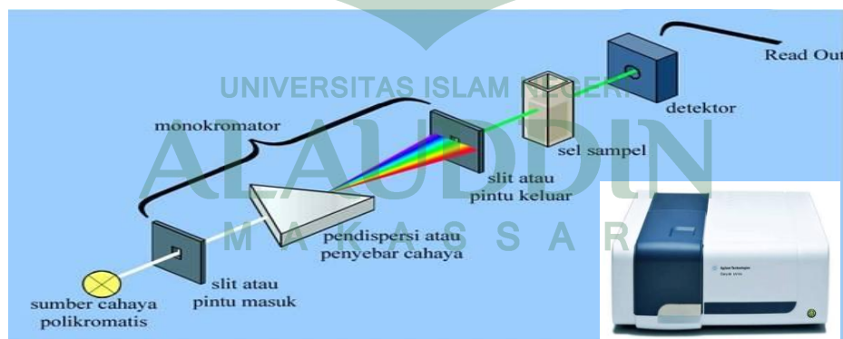
Gambar 2.1 Instrumen Spektrofotometer UV-Visible (Jannah: 2014)
