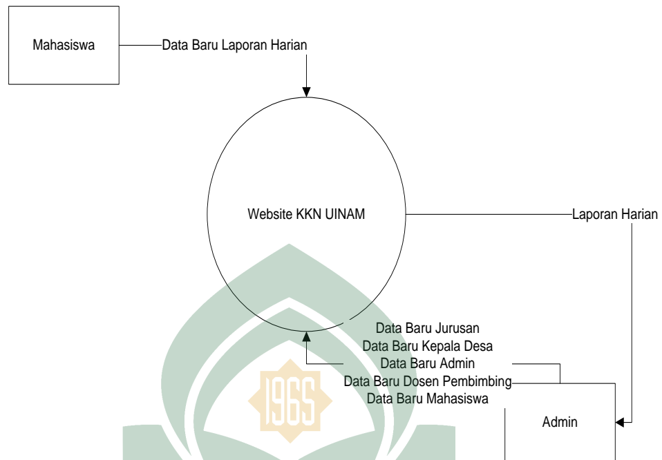
Gambar IV. 10. Diagram Konteks ( Level 0 )
