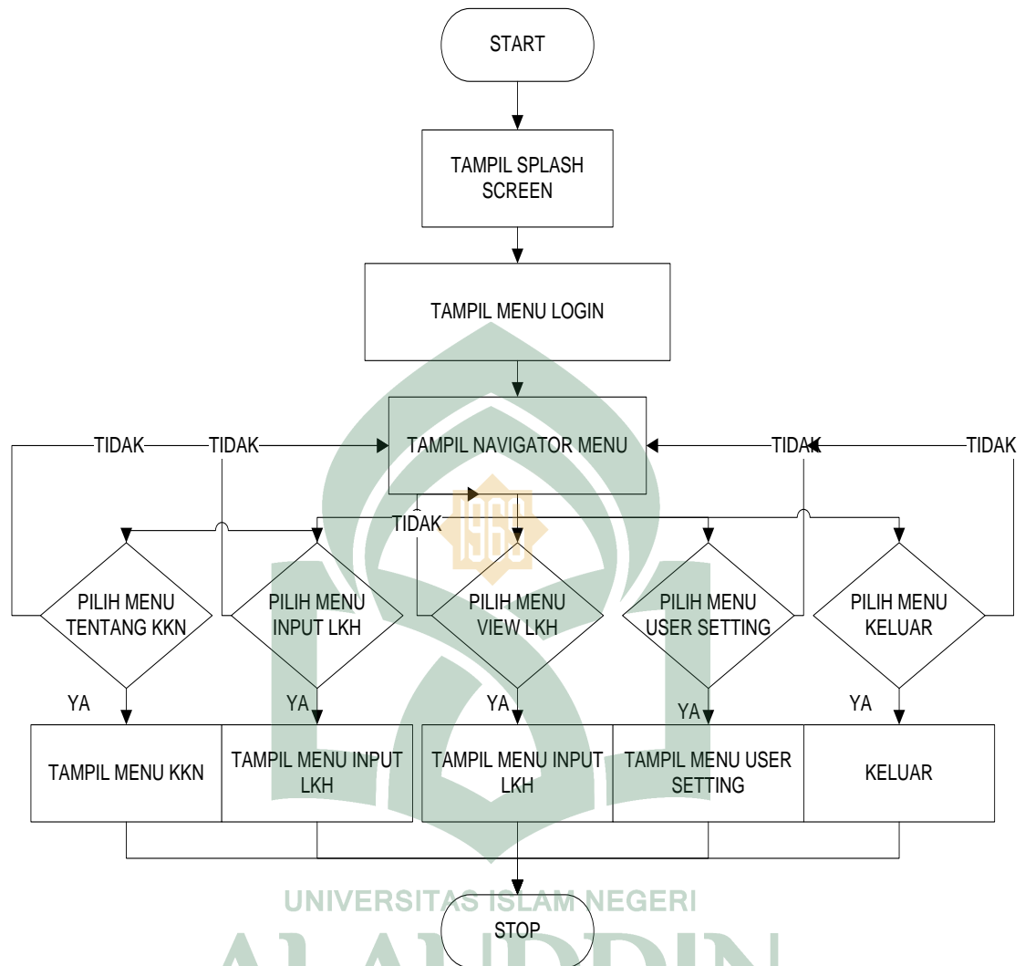
Gambar IV. 12 flowchart Android
