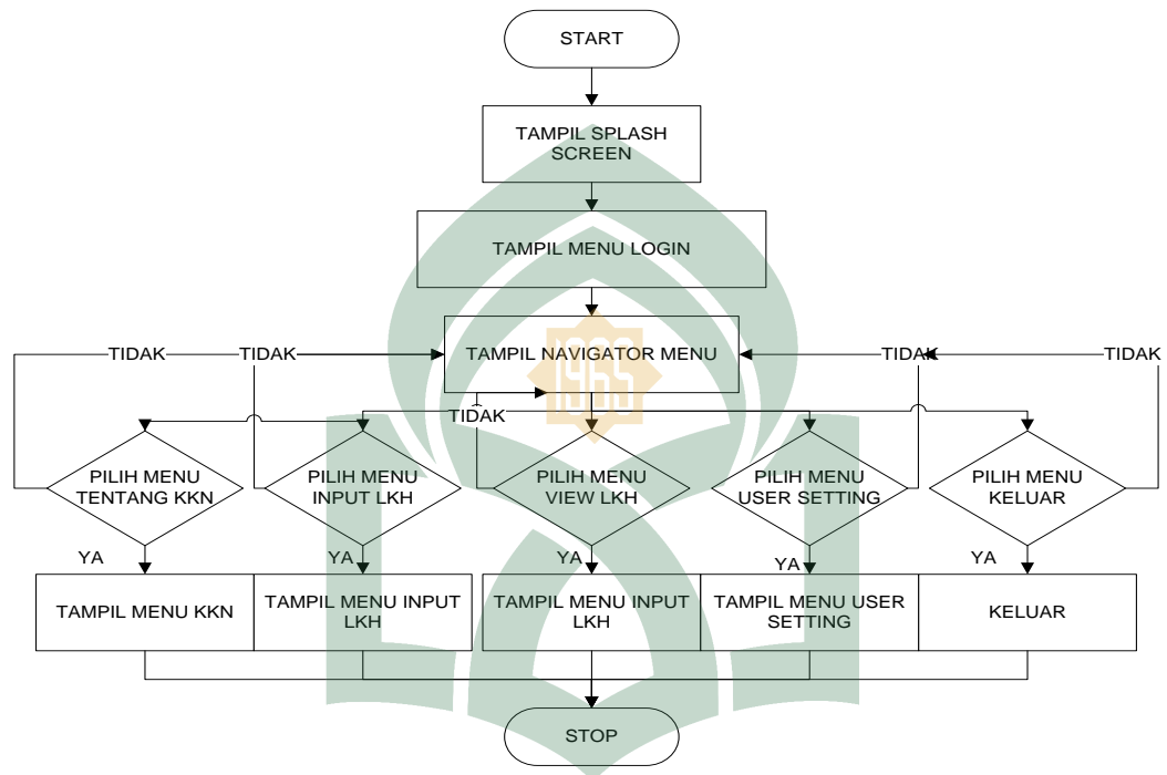
Gambar V.10 Flowchart Android
