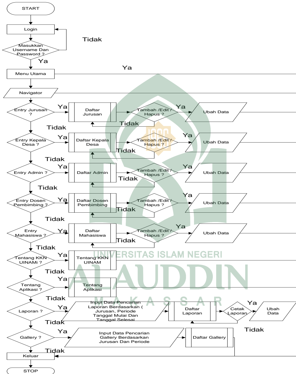
Gambar V.12 Flowchart Web
