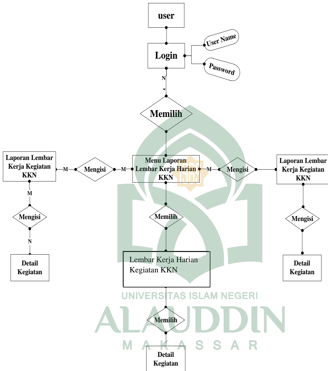
Gambar IV.11 Entity Relationship Diagram (ERD)
