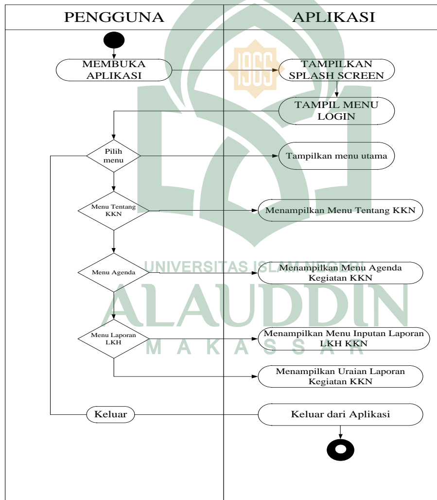
Gambar IV.7 Activity Diagram
