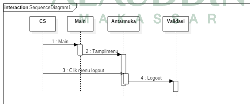
Gambar VI. 6 Sequence Diagram Menu Logout
