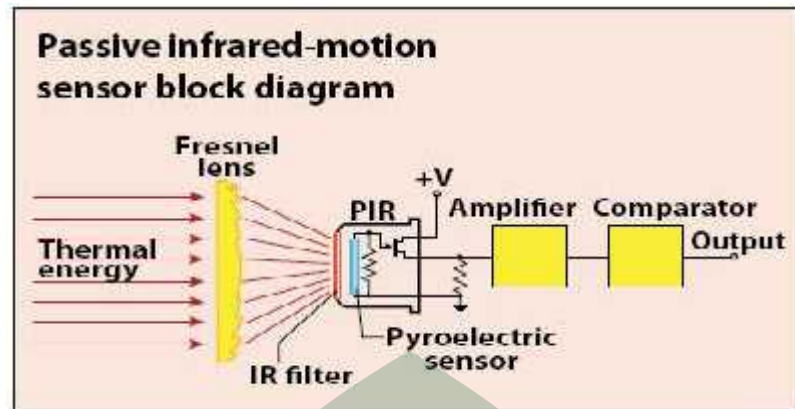
Gambar II.5. Blok Diagram Sensor PIR.
