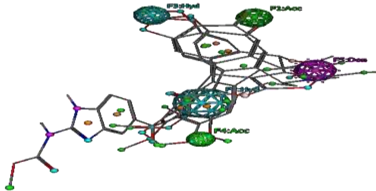
Gambar IV.4. Query farmakofor
