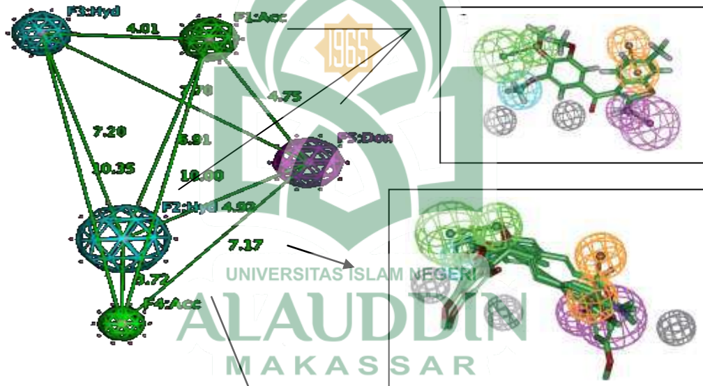
Gambar IV.4. Query farmakofor
