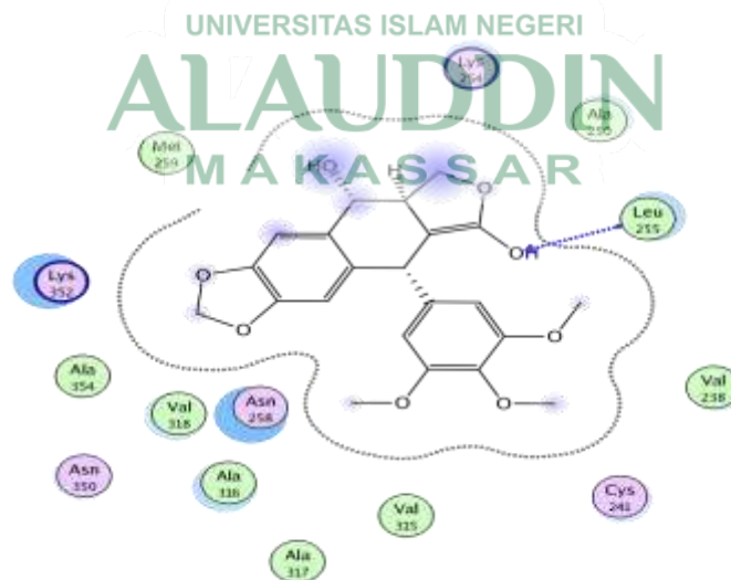
Gambar IV.3. Interaksi validasi ligan asli protein 1SA1
