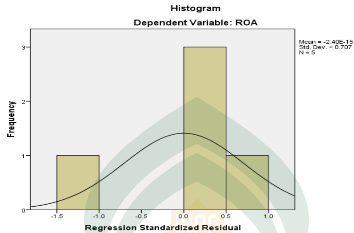
Gambar 4.1 Histogram
