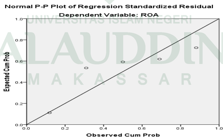
Gambar 4.2 Normal P-Plot
