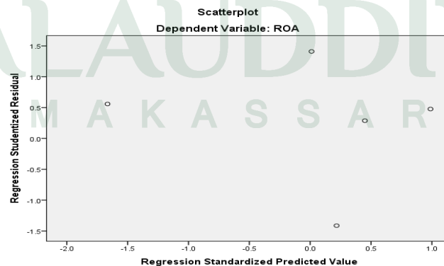
Gambar 4.3 Scatterplot
