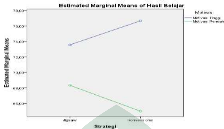
Gambar 4.2. Diagram Plot Antar Variabel
