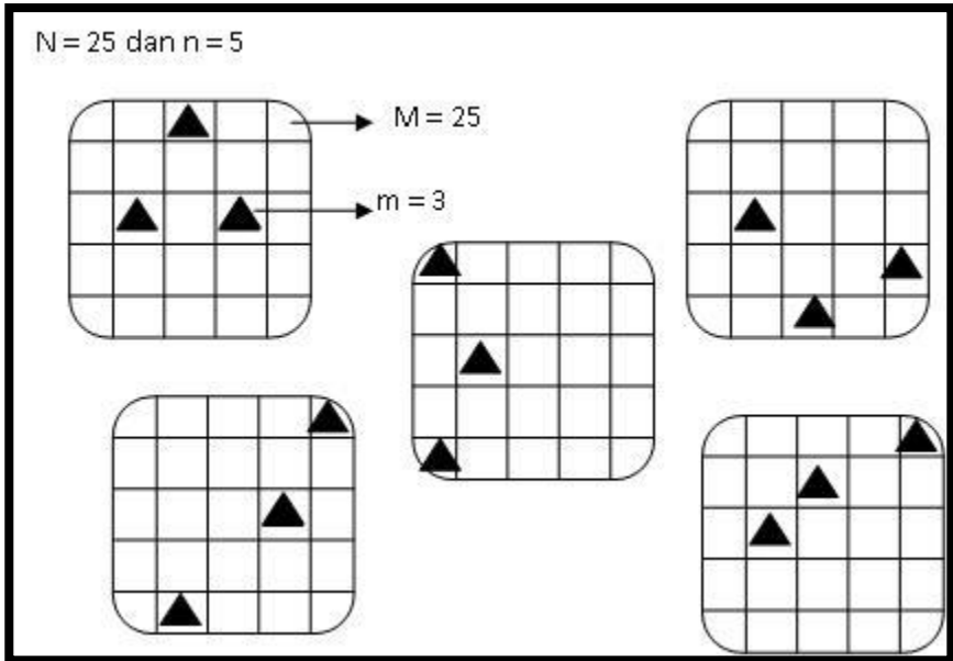
Gambar 5.3. Sampling Cluster Dua Tahap ( Two-Stage Cluster Sampling )
