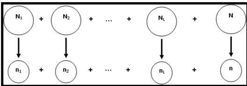
Gambar 5.2. Ilustrasi Sampling Berstrata ( Stratified Sampling )
