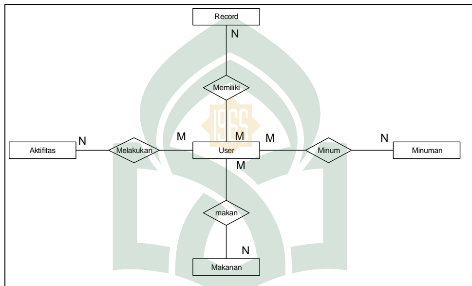
Gambar IV. 7. Entity Relationship Diagram (ERD)
