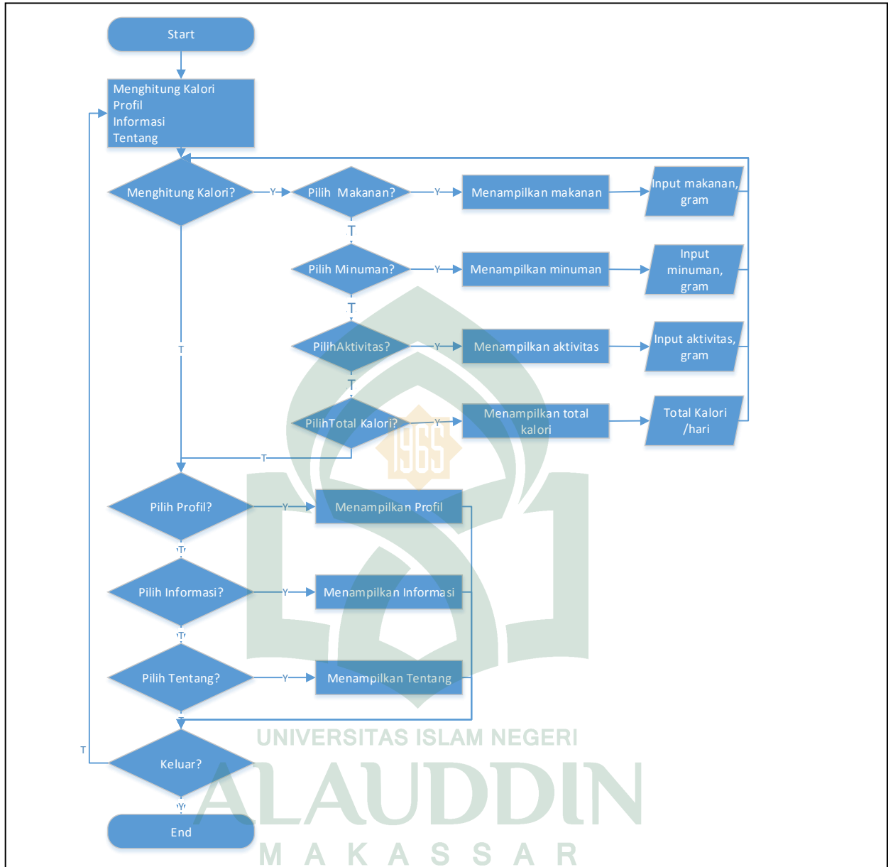
Gambar IV. 8. Flowchart
