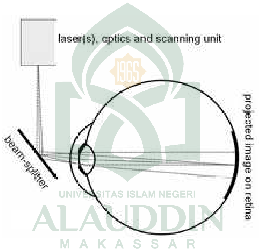
Gambar 2.6 Diagram sederhana virtual retina display Sumber: Thomas (2010)
