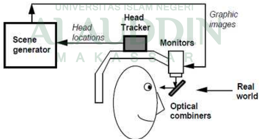
Gambar 2.4 Diagram see-through HMD Sumber: Paul M.(2007)
