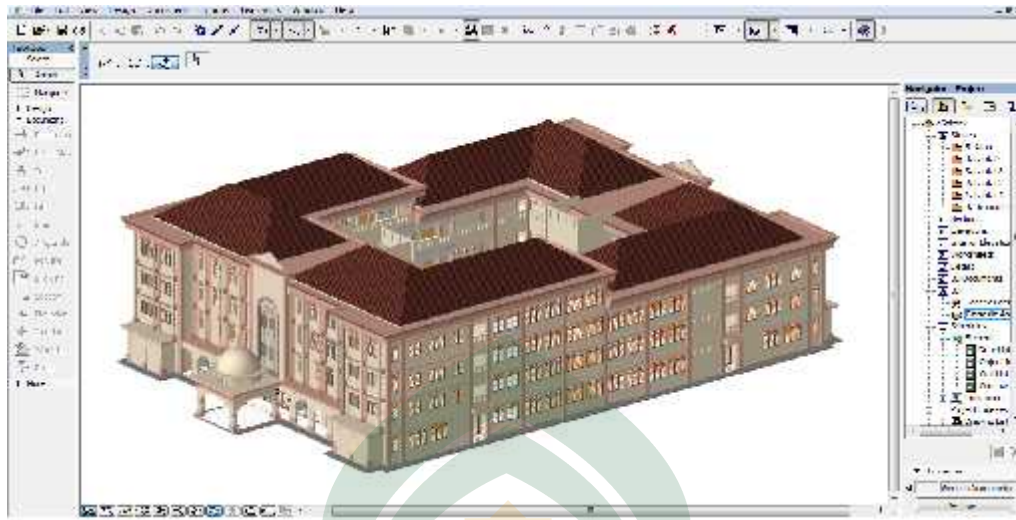
Gambar 4.7 Tampilan desain 3D Gedung Sainstek Tampak Axonometry.
