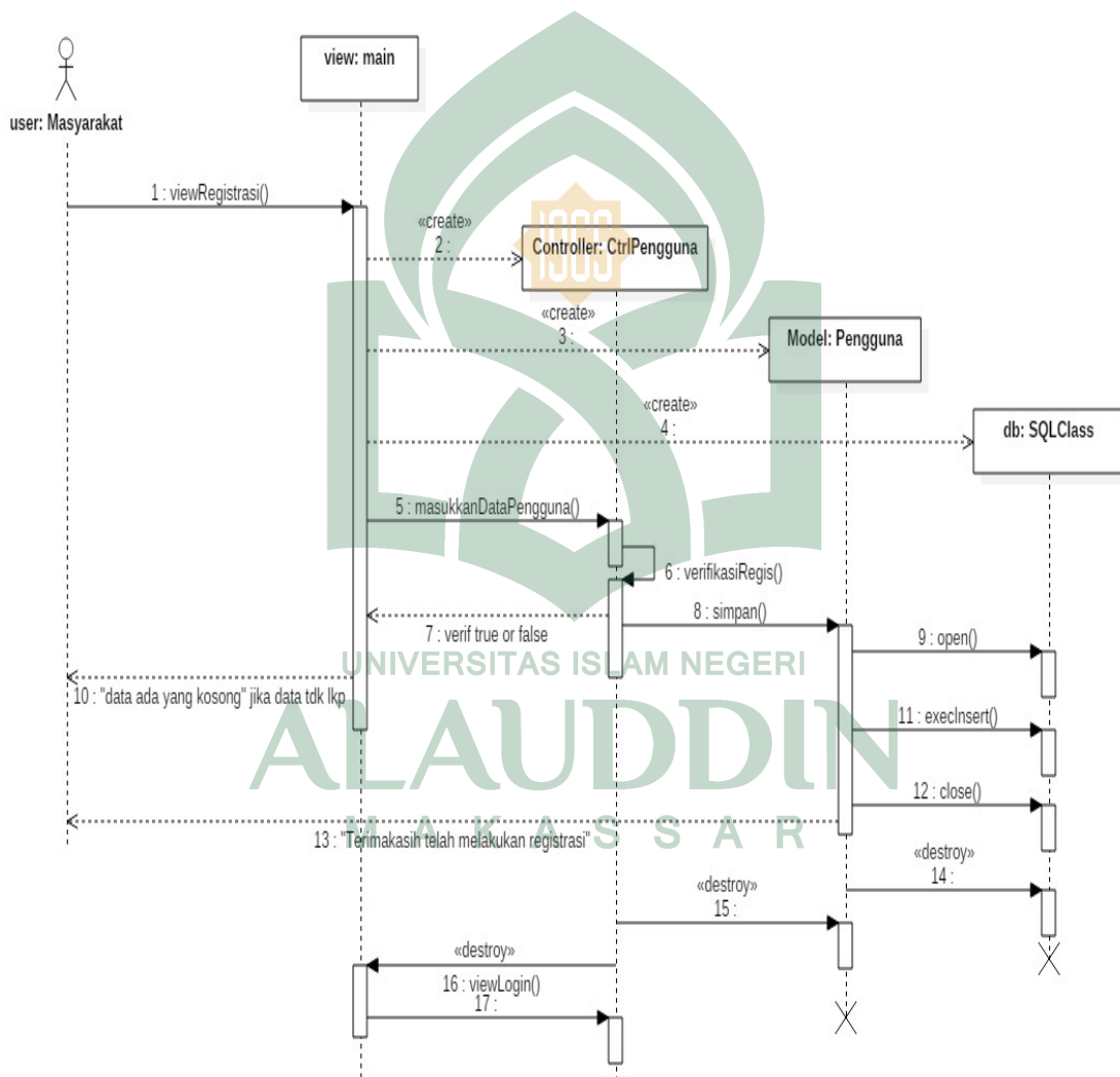
Gambar IV.6 Sequence Diagram Menu Registrasi
