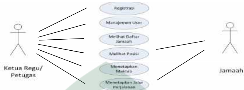
Gambar IV. 2 Diagram Use Case
