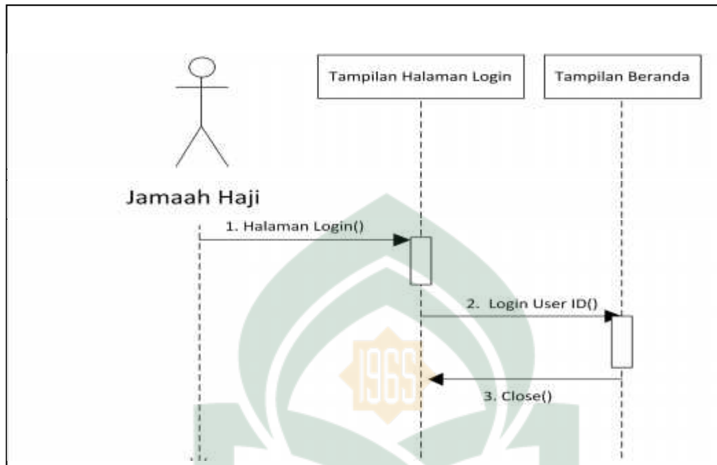
Gambar IV. 5 Diagram Sequence Jamah Haji
