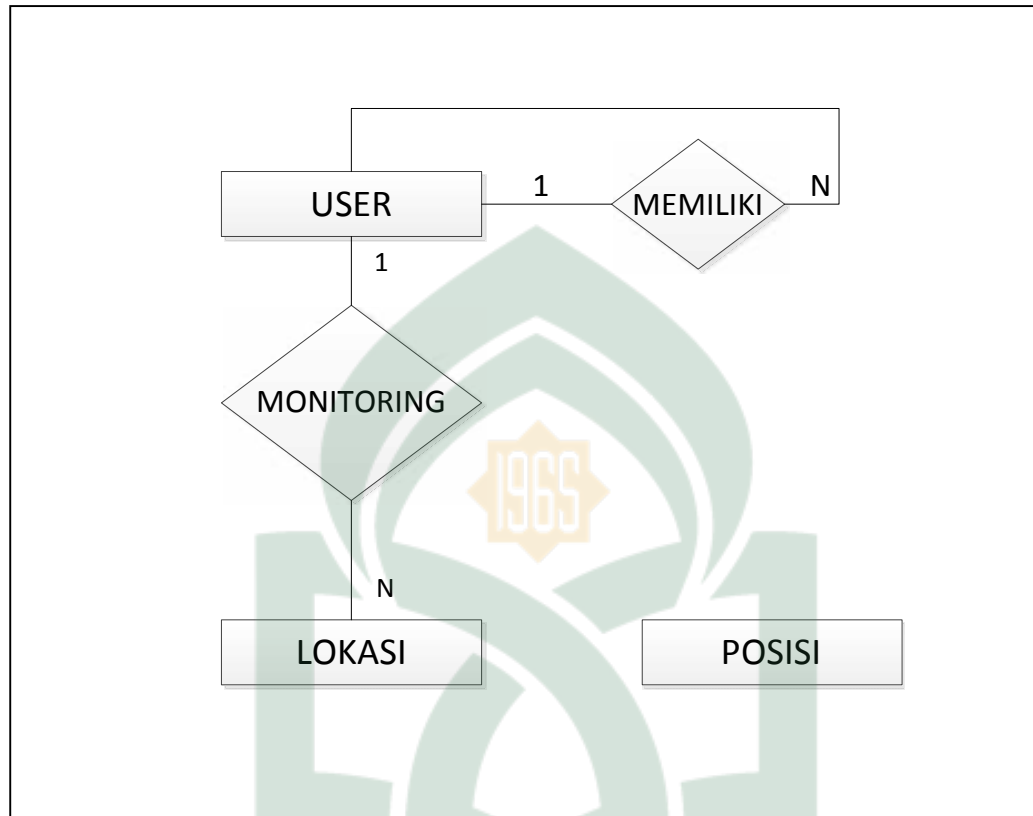
Gambar IV. 7 Entity Relationship Diagram
