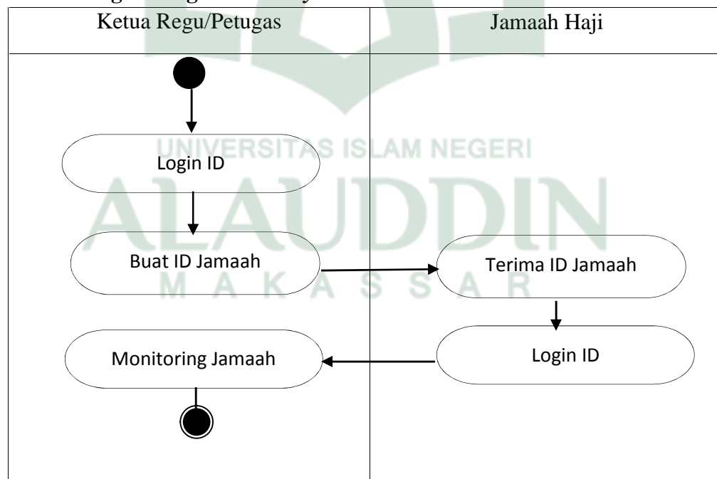
Gambar IV. 6 Diagram Activity
