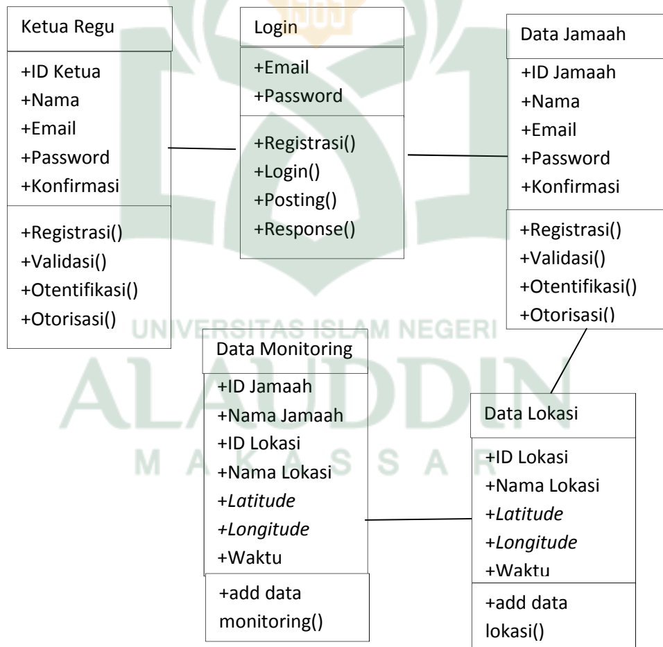
Gambar IV. 3 Diagram Class
