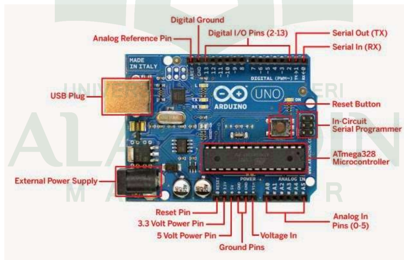
Gambar II.4 Bagian-Bagian Arduino UNO (Margolis, 2011)
