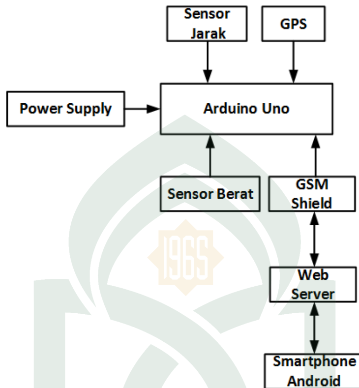
Gambar IV.2 Diagram blok Sistem Smart Trash Can berbasis Android
