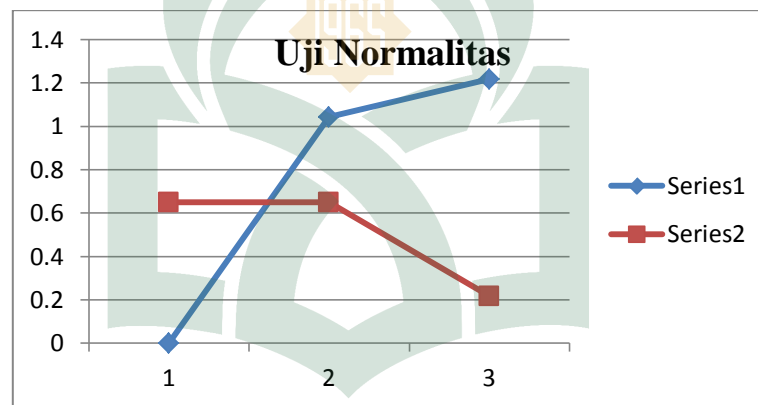
Gambar 4.3: Diagram Garis Uji Normalitas
