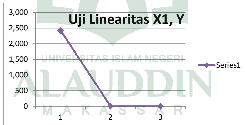
Gambar 4.4: Diagram Garis Uji Linieritas X1,Y
