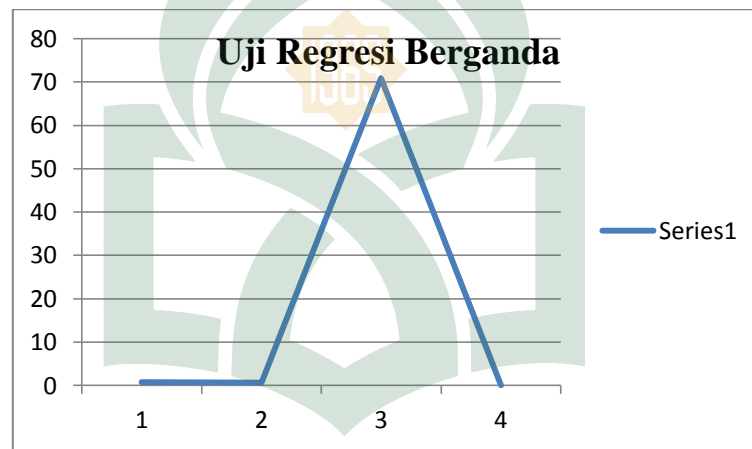
Gambar 4.6: Diagram Garis Hasil Analisis Regresi Berganda
