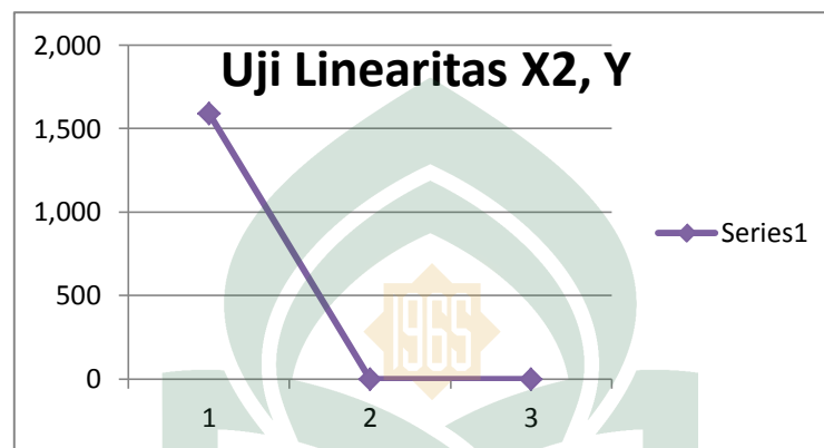
Gambar 4.5 : Diagram Garis Uji Linearitas X2, Y
