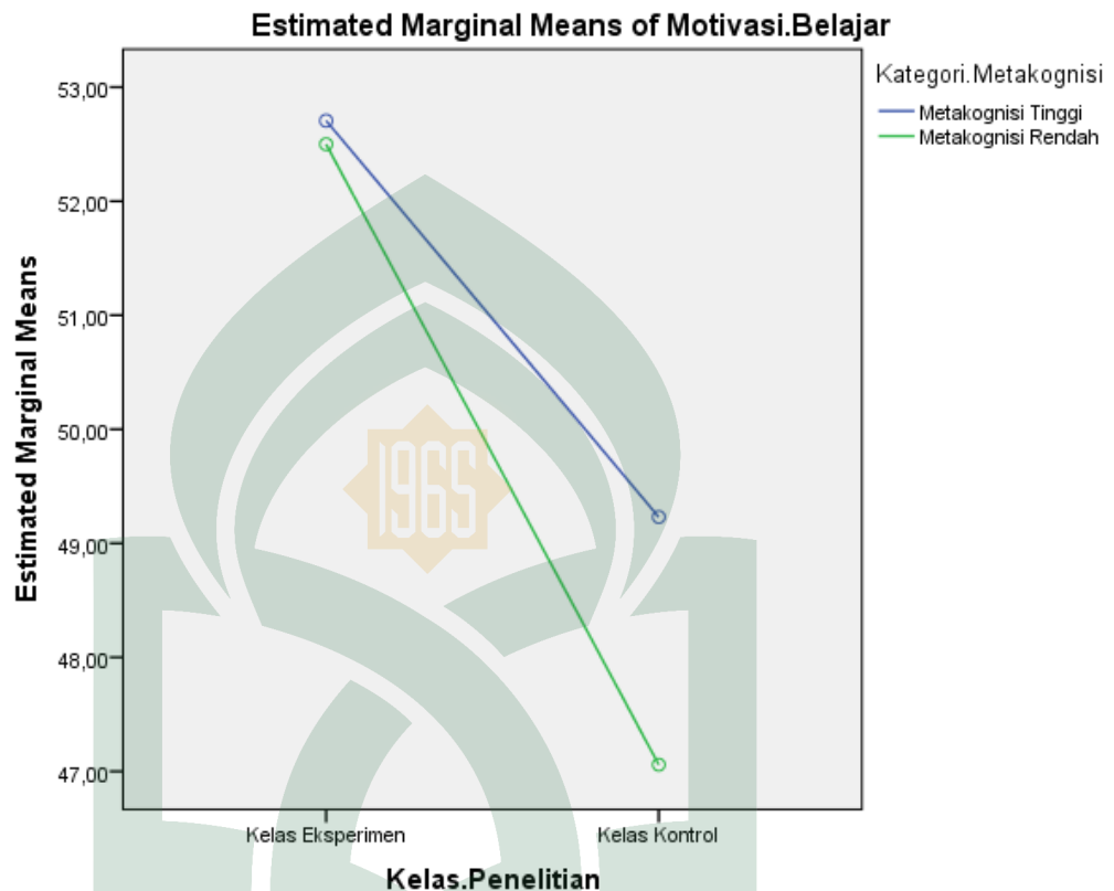
Gambar 4.2: diagram plot antar variabel
