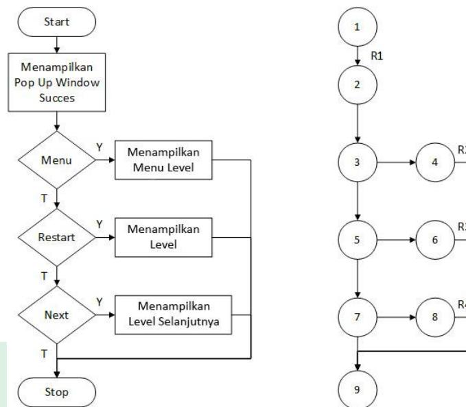
Gambar V.9 Flowchart dan Flowgraph Pop Up Window Success
