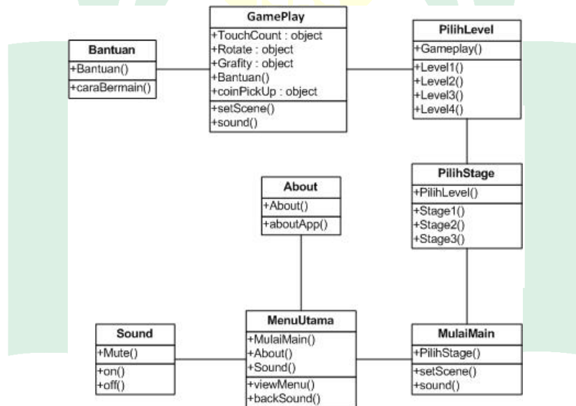
Gambar IV.4 Class Diagram Game Fun with Physic
