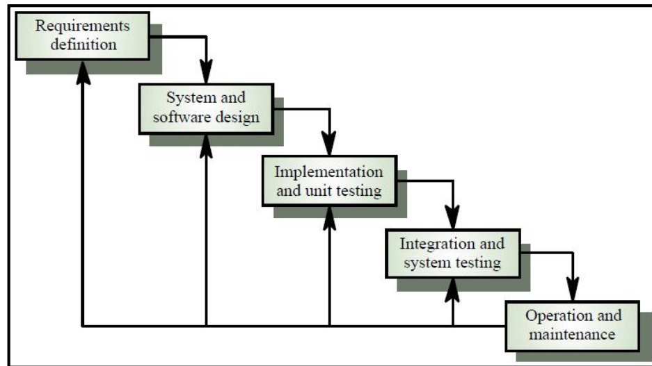
Gambar III.1 Metode Waterfall
