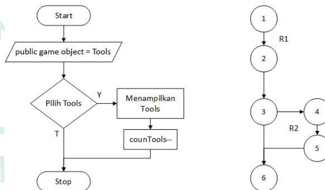
Gambar V.11 Flowchart dan Flowgraph Tools
