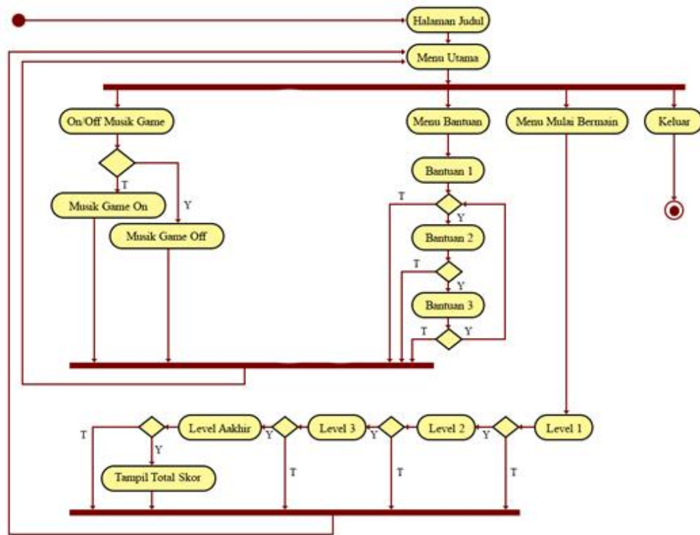
Gambar IV.8 Activity Diagram
