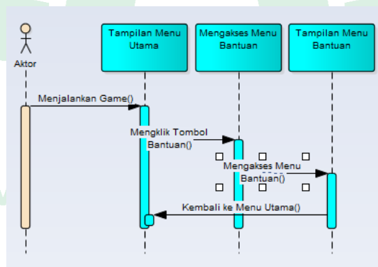
Gambar IV.7 Sequence Diagram Melihat Bantuan
