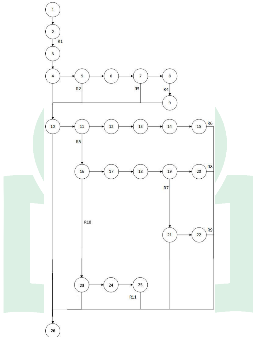
Gambar V.13 Flowgraph Flowchart Drag dan Rotate Tools
