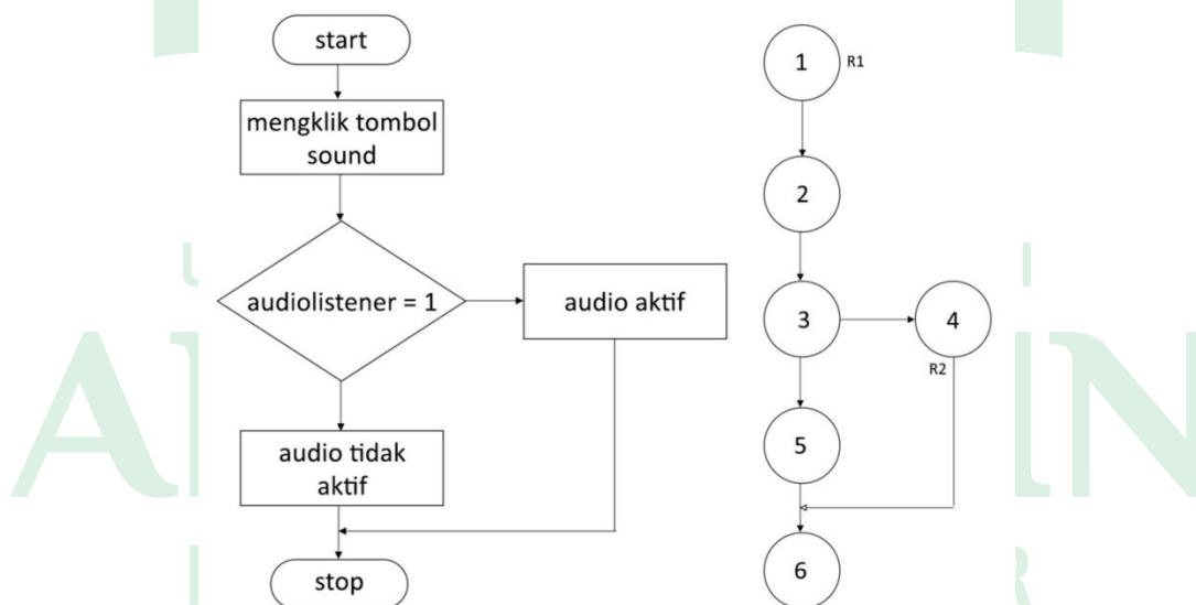
Gambar V.14 Flowgraph Flowchart On dan Off Sound
