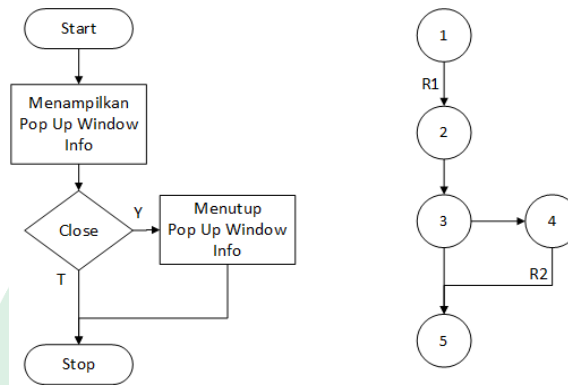
Gambar V.10 Flowchart dan Flowgraph Pop Up Window Info
