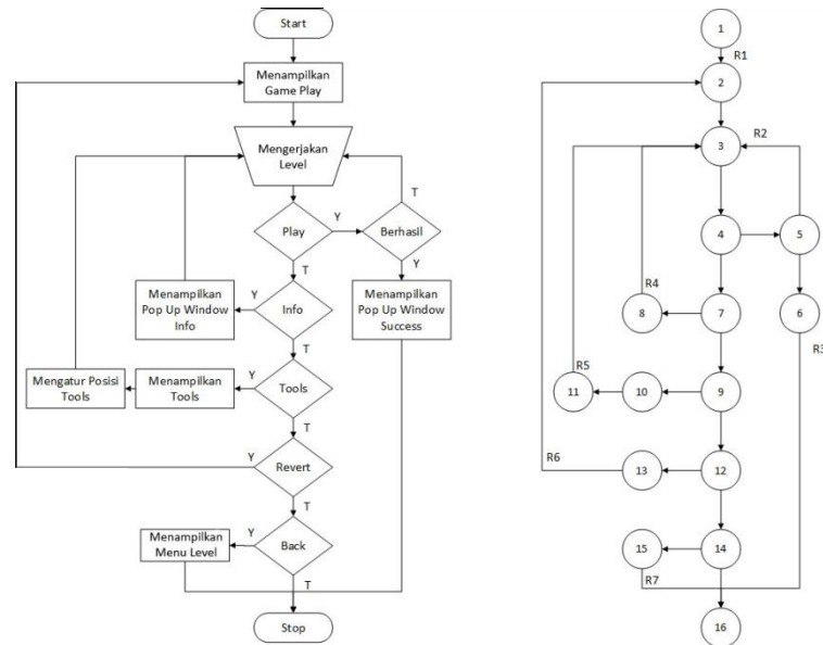
Gambar V.8 Flowchart dan Flowgraph Stage
