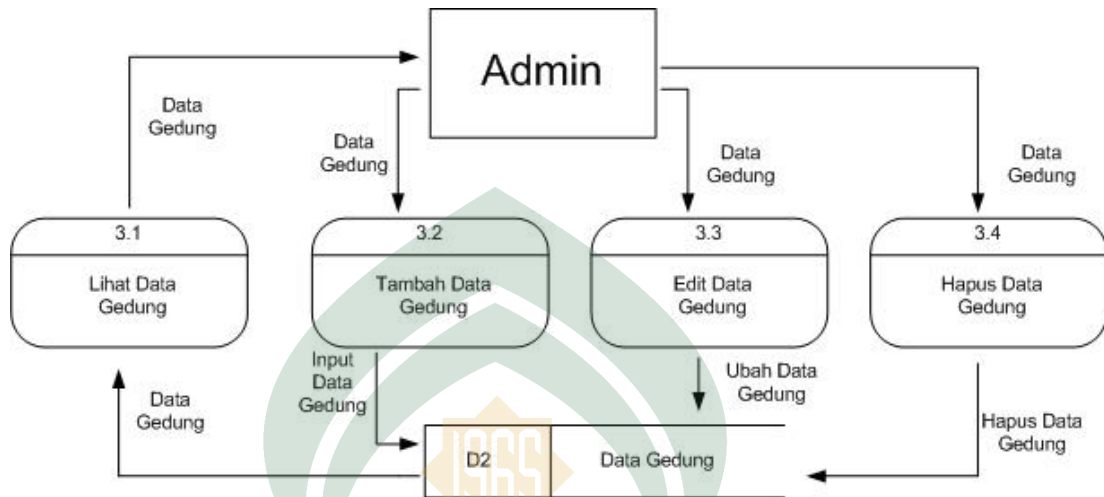
Gambar IV.13 Arus Data Level 1 Proses 3
