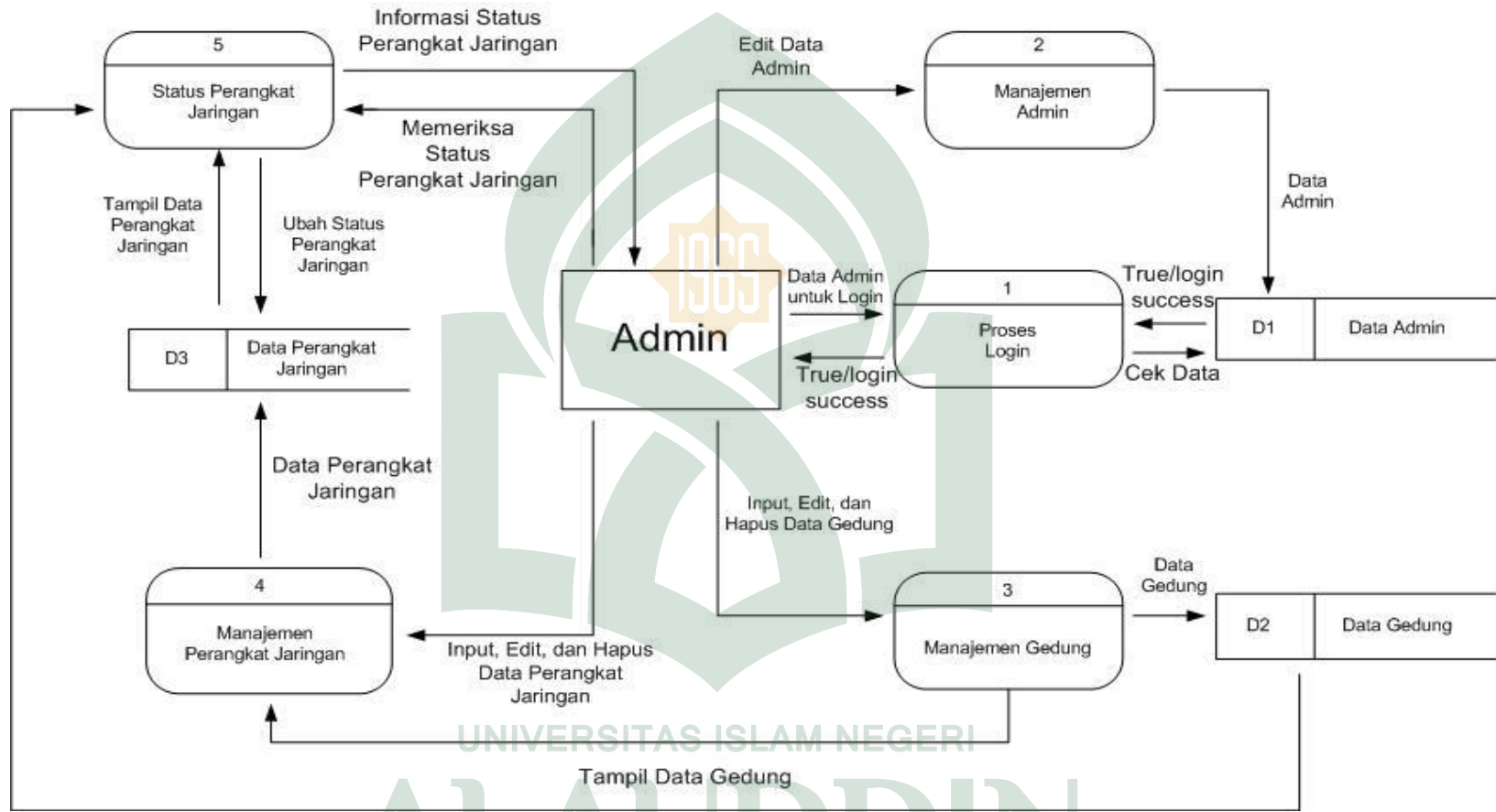
Gambar 4.10 Arus Data Level 0
