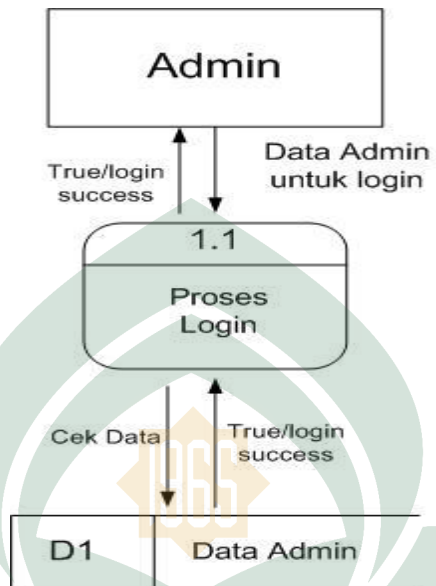
Gambar IV.11 Arus Data Level 1 Proses 1
