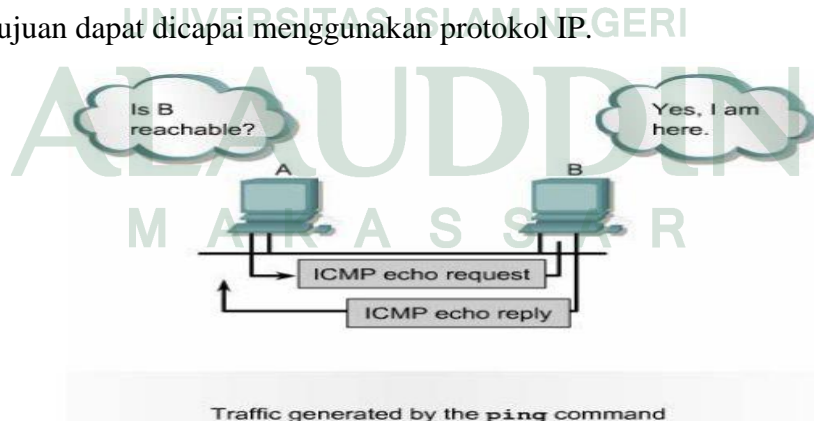
Gambar 2.4 Echo Reply
