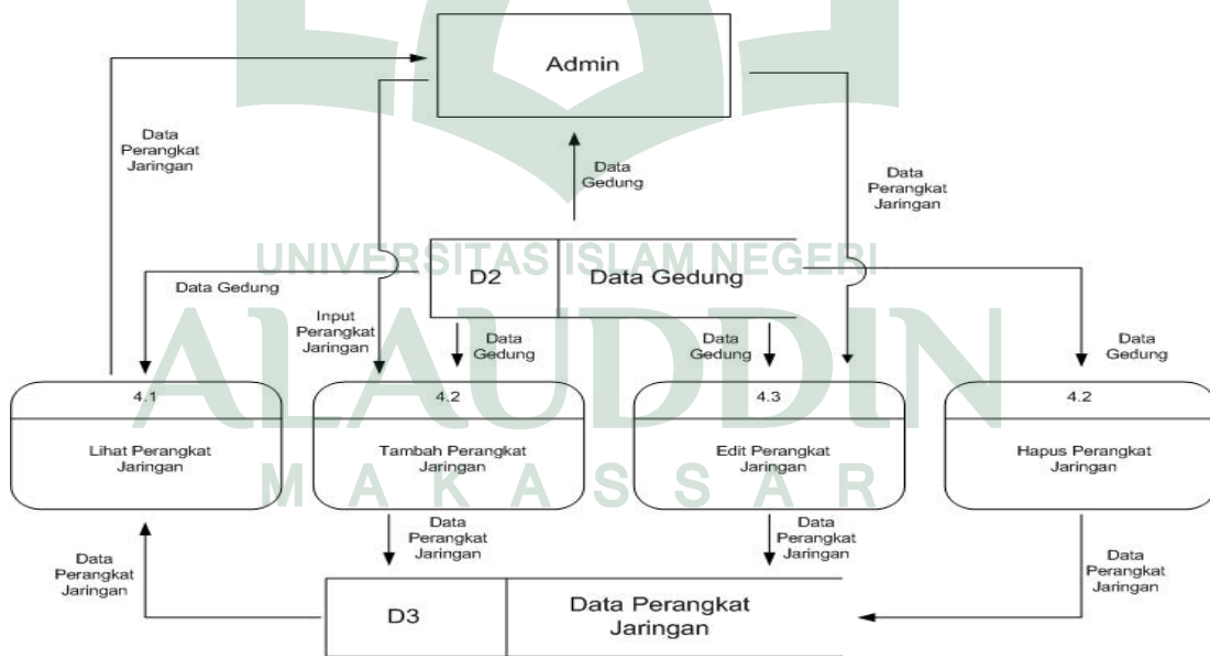
Gambar 4.14 Diagram Arus Level 1 Proses 4
