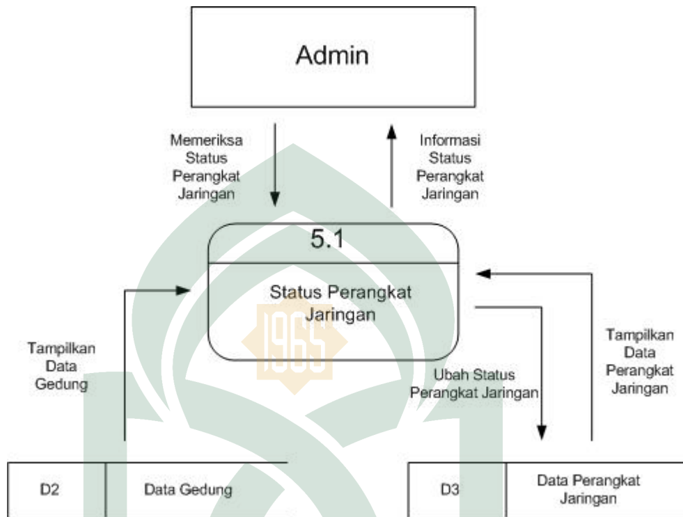
Gambar 4.15 Diagram Arus Level 1 Proses 5
