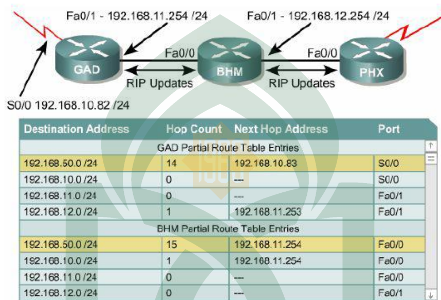
Gambar 2.6 Hop Count
