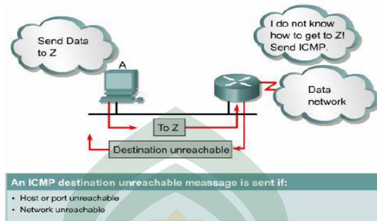
Gambar 2.3 Destination unreachable
