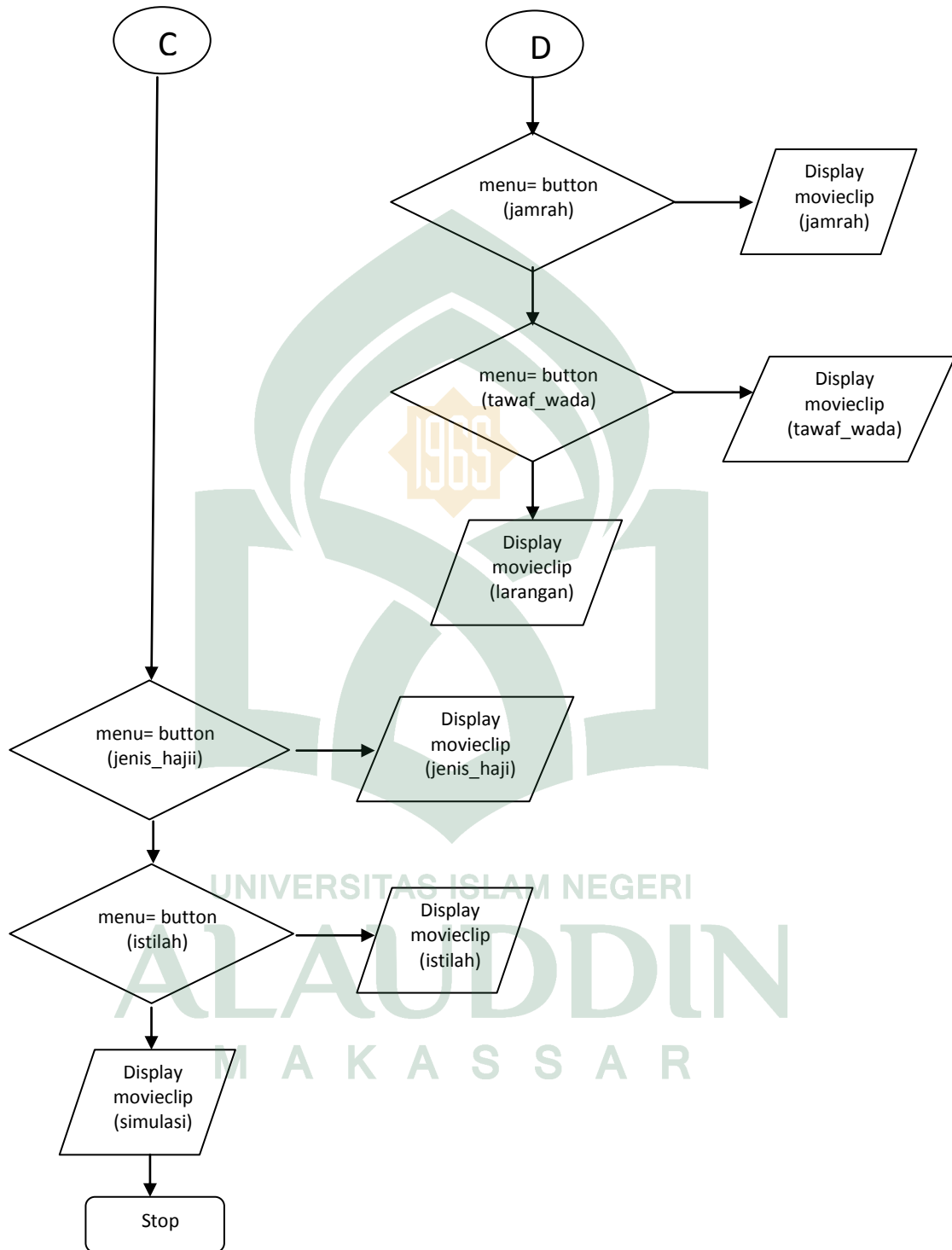
Gambar IV.5 Flowchart Program
