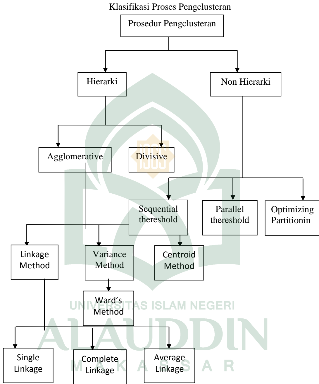
Gambar2.1 Bagan Analisis Cluster 7
