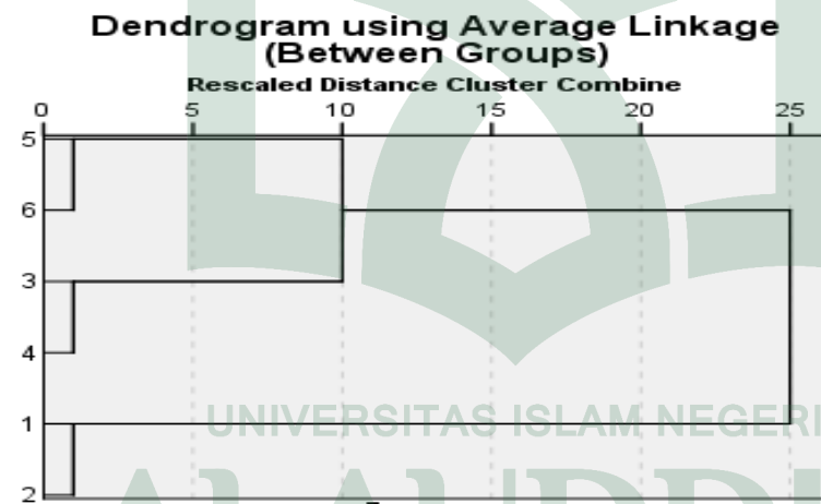
Gambar. 2.2. Contoh Dendrogram Average Linkage
