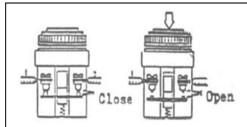
Gambar II.5: Push button tipe NC
