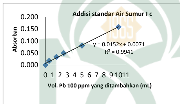
Gambar 4. Kurva addisi standar sumur 1 (c)
