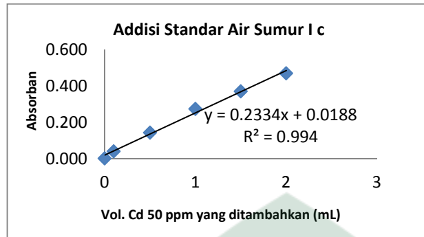
Gambar 14. Kurva addisi standar sumur 1 (c)
