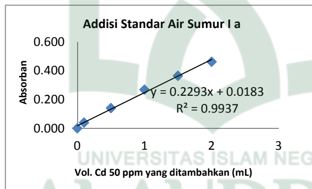
Gambar 12. Kurva addisi standar sumur 1 (a)
