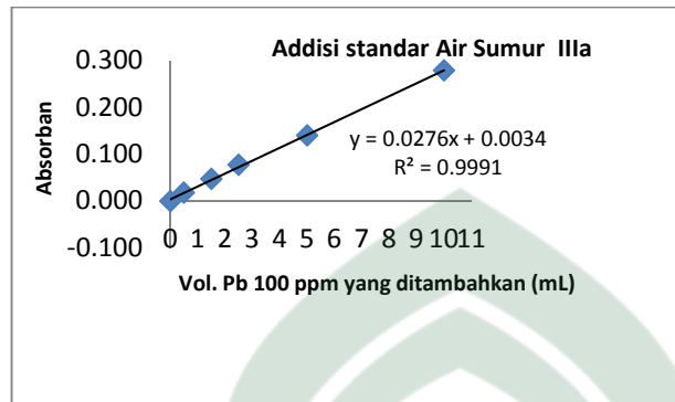
Gambar 8. Kurva addisi standar sumur 3 (a)
