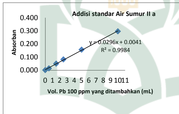
Gambar 5. Kurva addisi standar sumur 2 (a)
