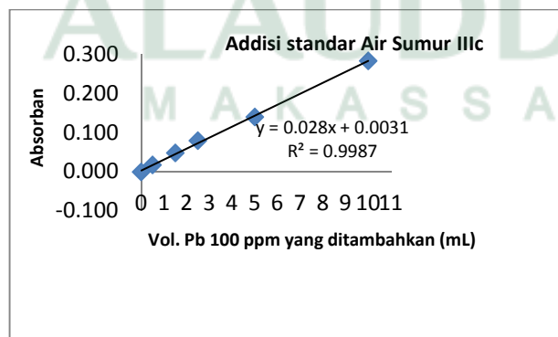
Gambar 10. Kurva addisi standar sumur 3 (c)
