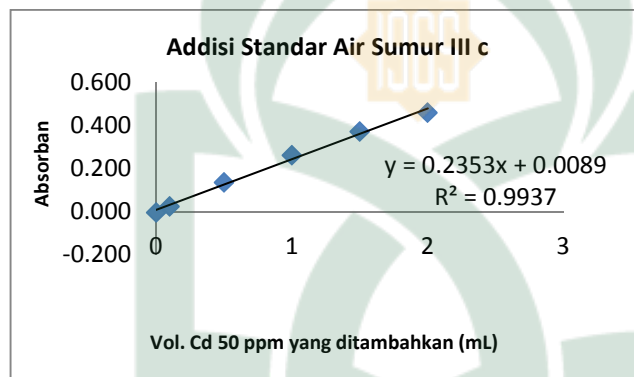
Gambar 20. Kurva addisi standar sumur 3 (c)
