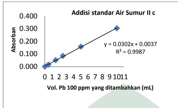
Gambar 7. Kurva addisi standar sumur 2 (c)
