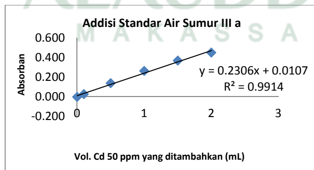
Gambar 18. Kurva addisi standar sumur 3 (a)
