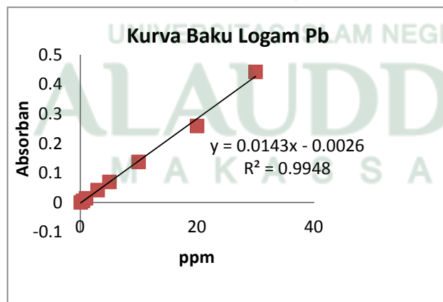
Gambar 1. Kurva baku logam Timbal (Pb)
