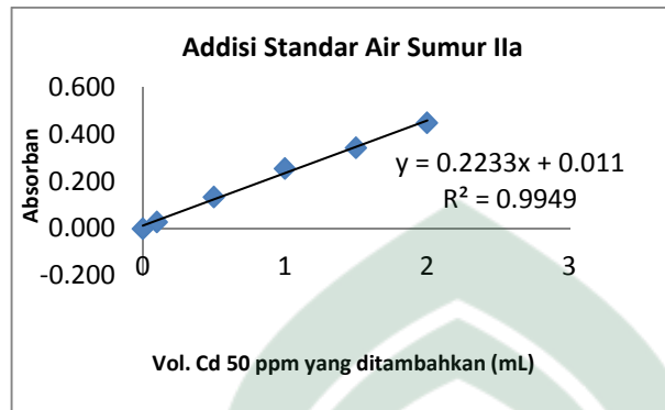
Gambar 15. Kurva addisi standar sumur 2 (a)
