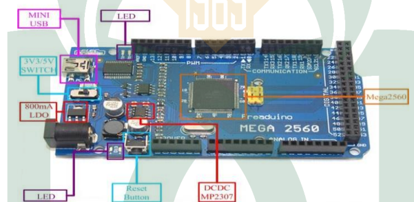
Gambar II.2 Arduino Mega 2560 (Oktariawan, 2015).
