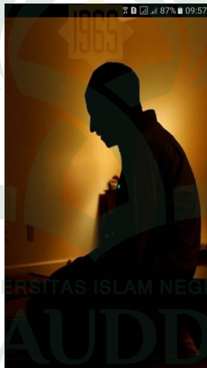
Gambar V.1 Antarmuka SplashScreen
