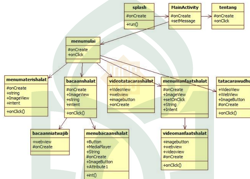
Gambar IV.4. Class Diagram
