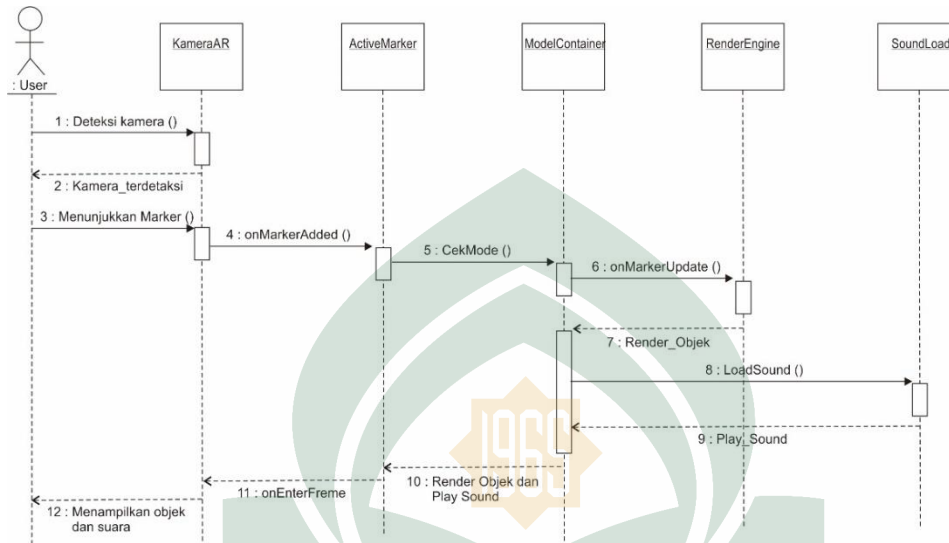
Gambar IV. 9 Sequence Diagram Menu Kamera AR
