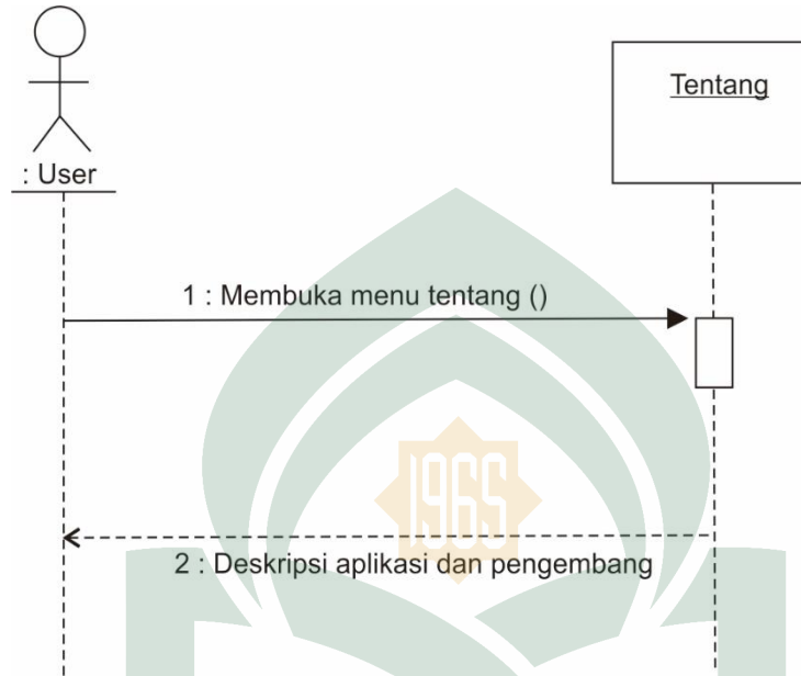
Gambar IV. 11 Sequence Diagram Menu Tentang
