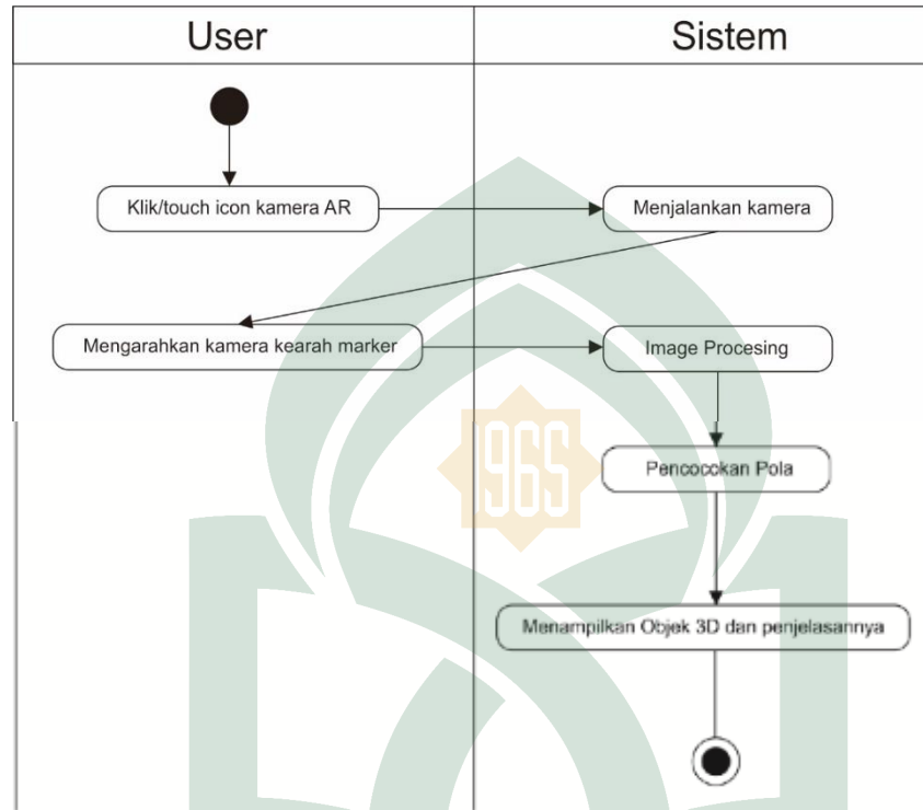
Gambar IV. 5 Activity Diagram Menu Kamera AR
