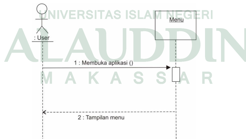
Gambar IV. 8 Sequence Diagram Menu
