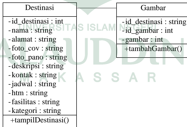
Gambar IV.4 Class Diagram
