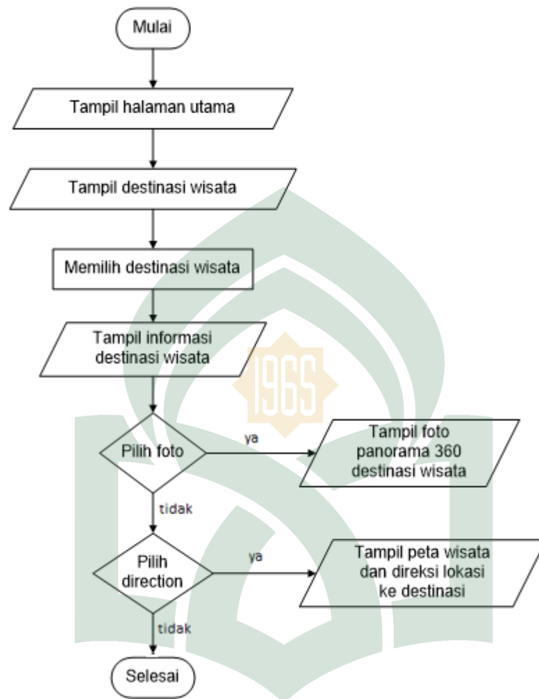
Gambar IV.9 Flowchart
