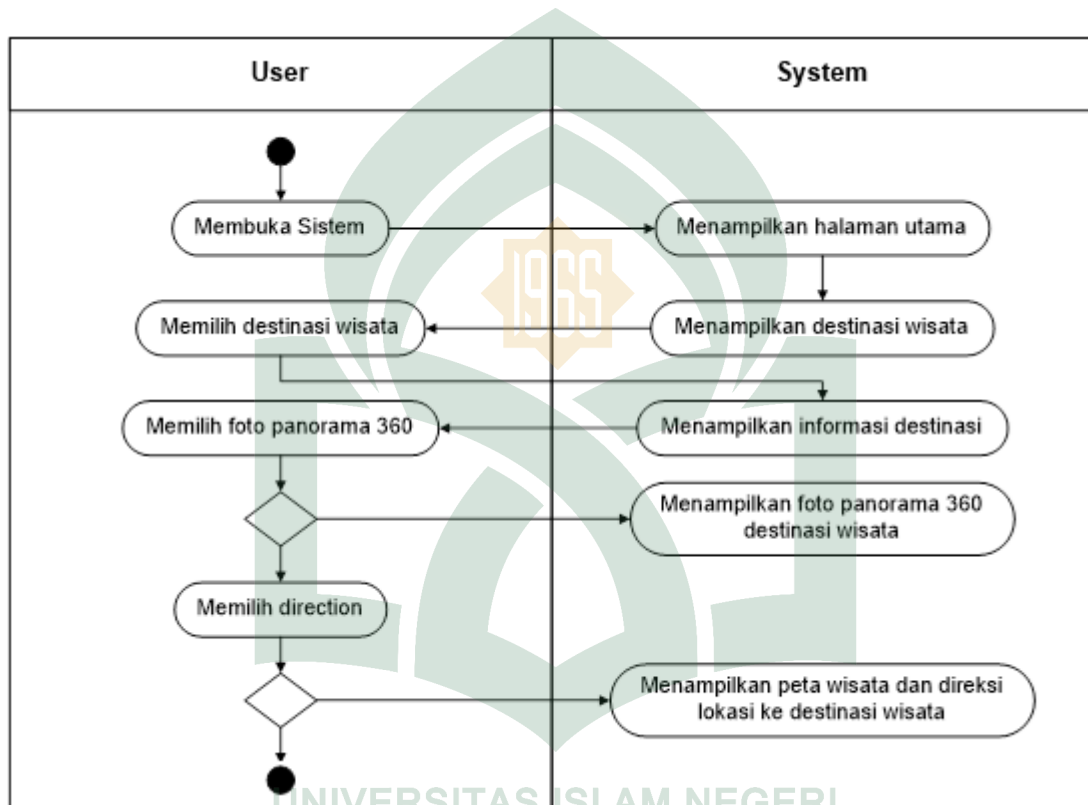
Gambar IV.8 Activity Diagram
