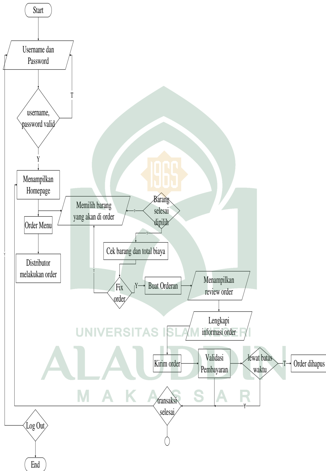
Gambar IV.14 Flowchart
