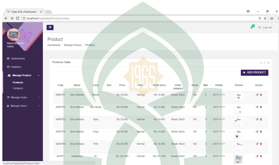
Gambar V.4 Antarmuka Products
