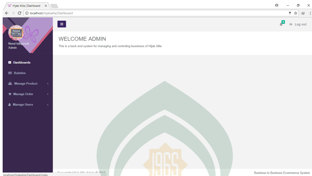
Gambar V.2 Antarmuka Dashboard
