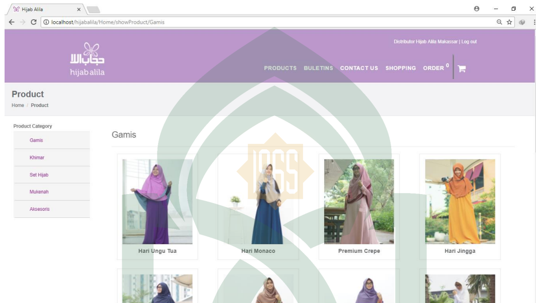
Gambar V.16 Antarmuka Product
