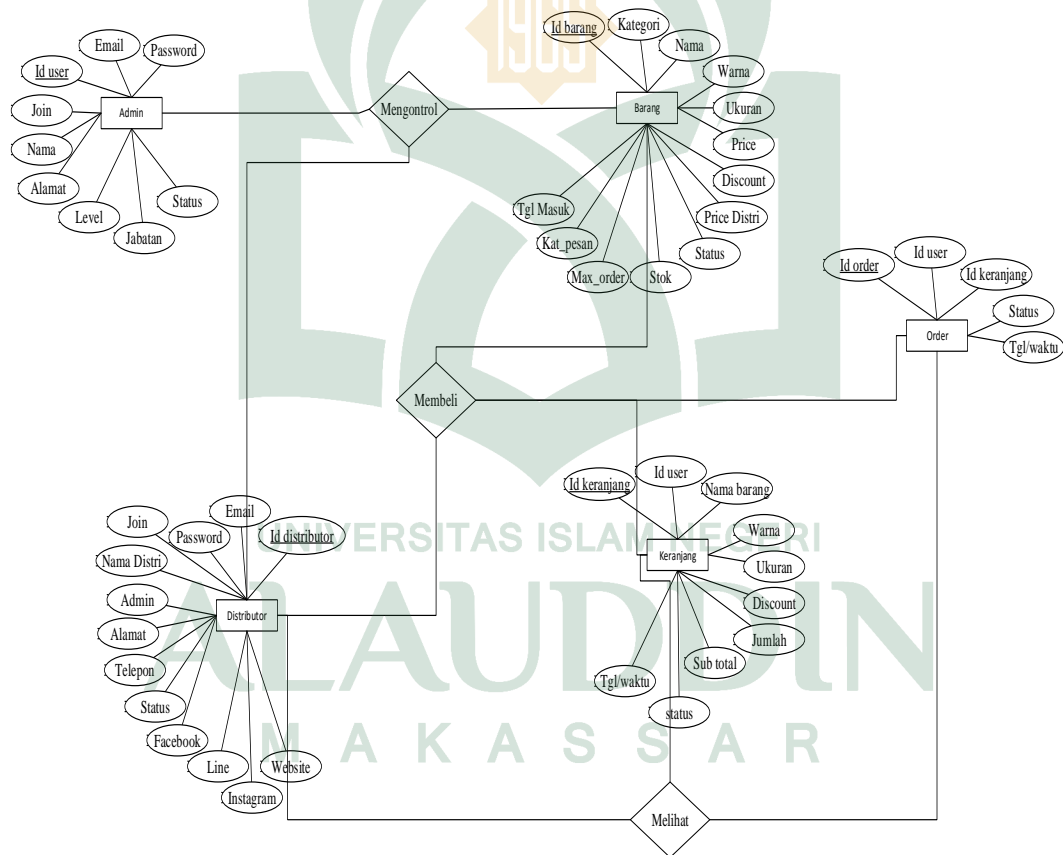
Gambar IV.23 Entitas Relationship Diagram
