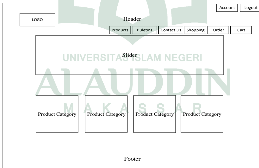
Gambar IV.16 Antarmuka Homepage
