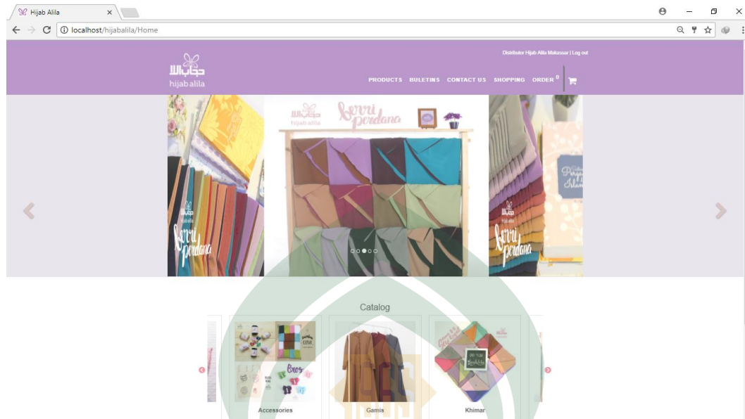
Gambar V.14 Antarmuka Homepage
