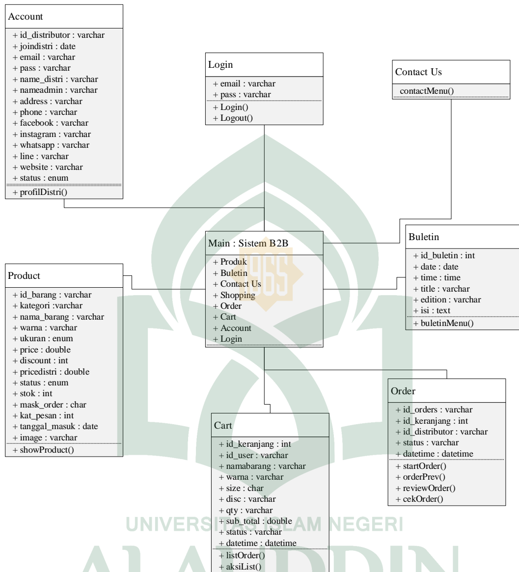
Gambar IV.4 Class Diagram
