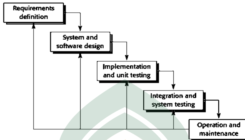
Gambar. III. 1 Model Waterfall
