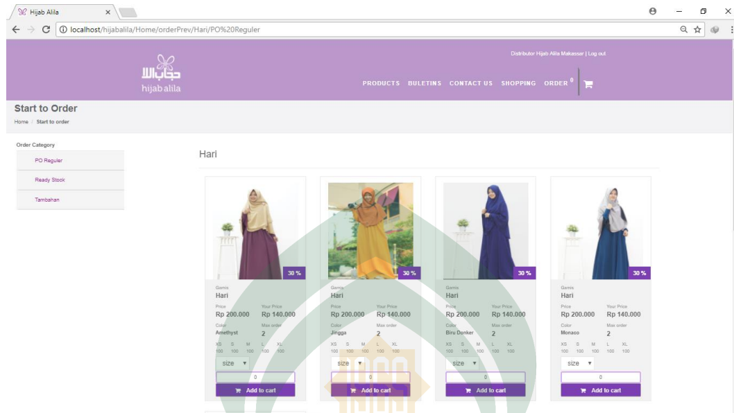
Gambar V.17 Antarmuka Shopping
