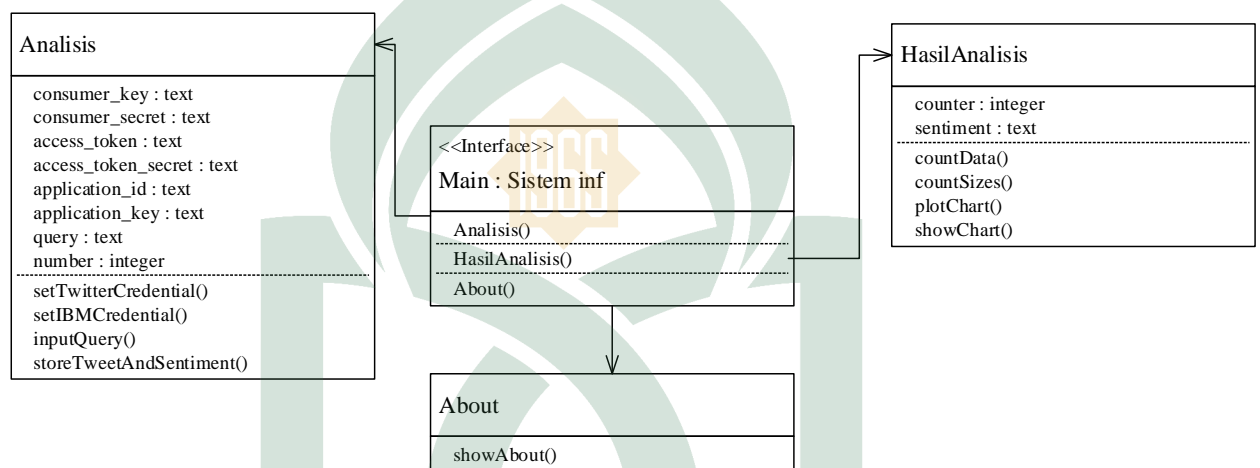
Gambar IV.4 Class Diagram
