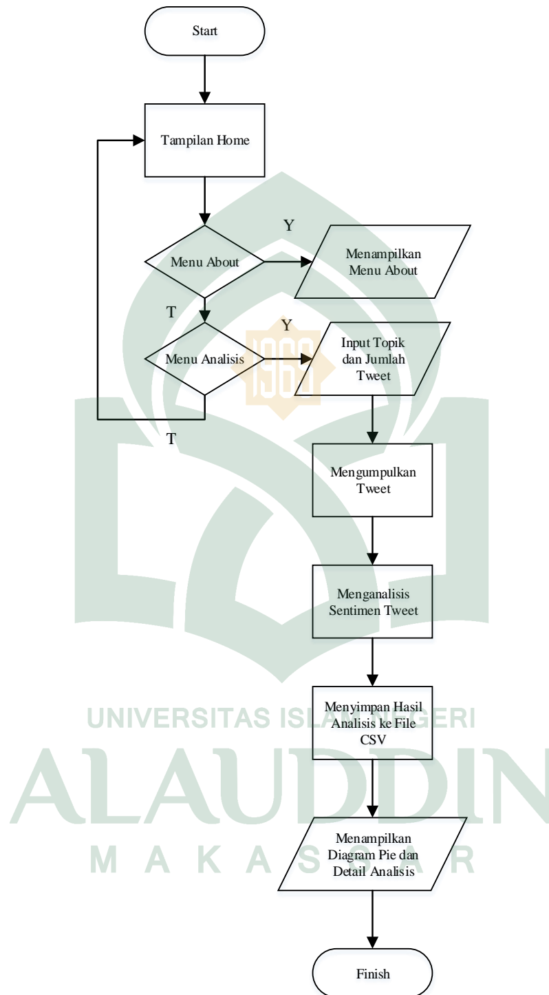
Gambar IV.8 Flowchart
