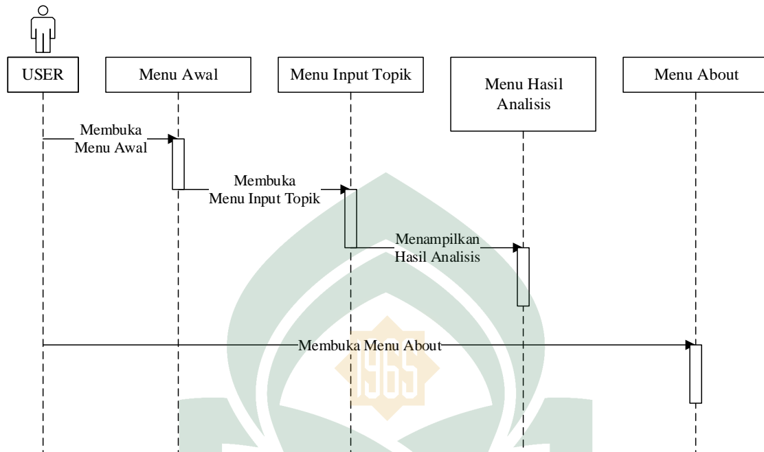
Gambar IV. 5 Squence Diagram
