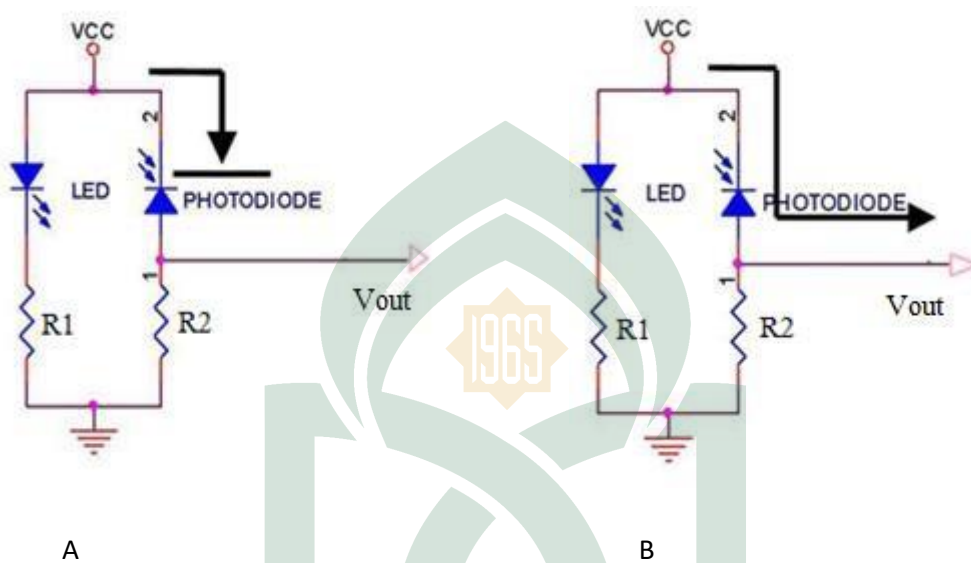
Gambar II.6 Rangkaian prinsip kerja sensor photodiode
