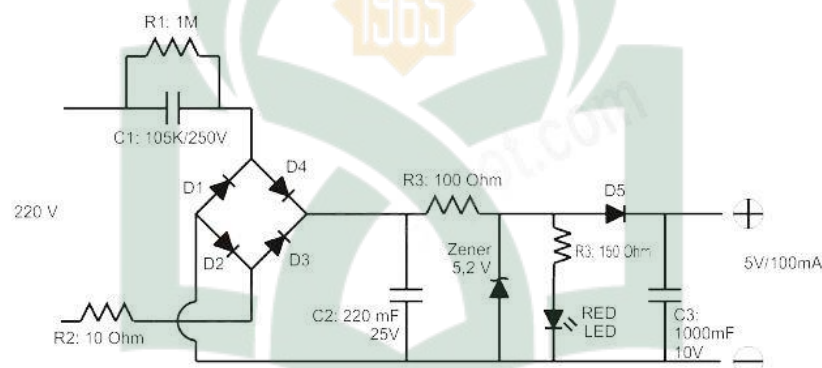
Gambar IV.5 Rangkaian Power Supply (Suhartono, 2015).
