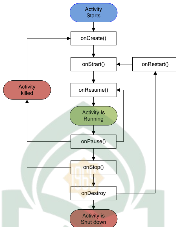
Gambar II.2 Bagan Daur Hidup Activity Android (Google, 2016)
