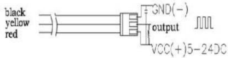
Gambar IV.6 Wiring Diagram Sensor Flow Meter. (Google, 2017)
