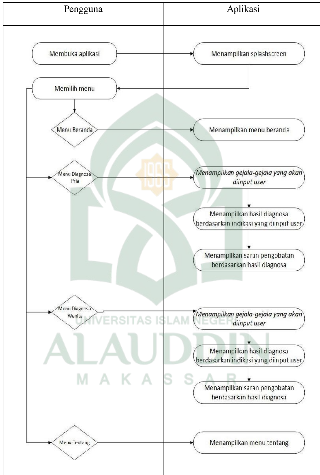
Gambar IV. 7 Activity Diagram
