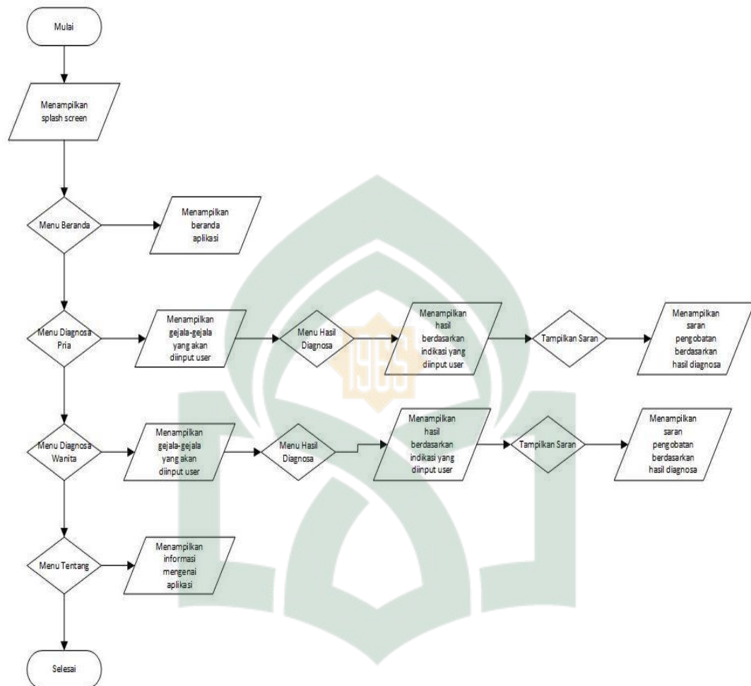
Gambar IV.9 Flowchart
