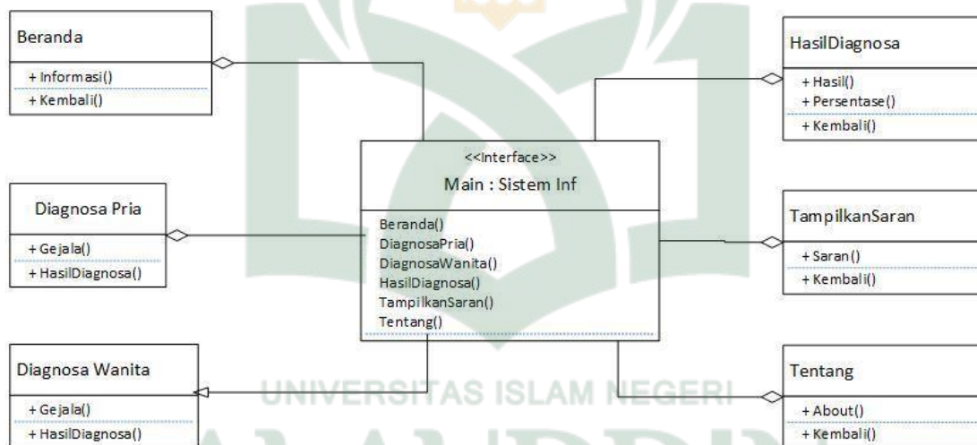
Gambar IV. 4 Class Diagram
