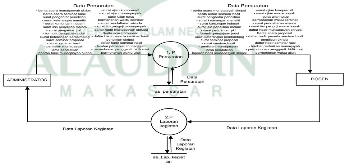
Gambar IV.5 Data flow diagram level 0
