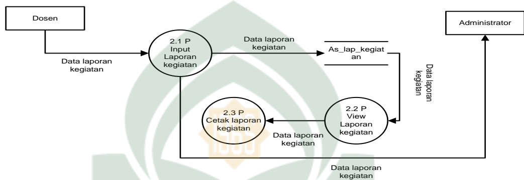
Gambar IV.7 Data Flow Diagram level 1 proses 2
