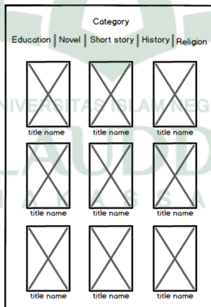
Gambar IV.18 Tampilan Category
