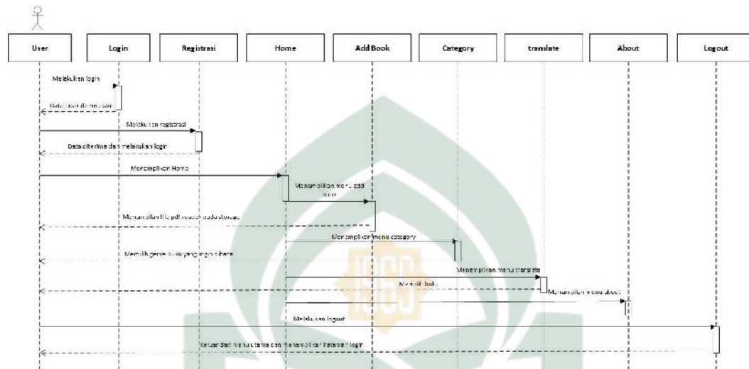
Gambar IV.5 Sequence Diagram User
