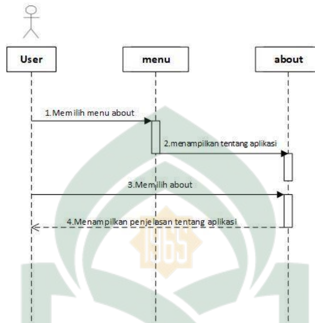
Gambar IV.9 Sequence Diagram About
