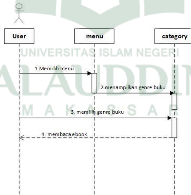
Gambar IV.6 Sequence Diagram Category
