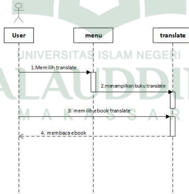
Gambar IV.8 Sequence Diagram Translate
