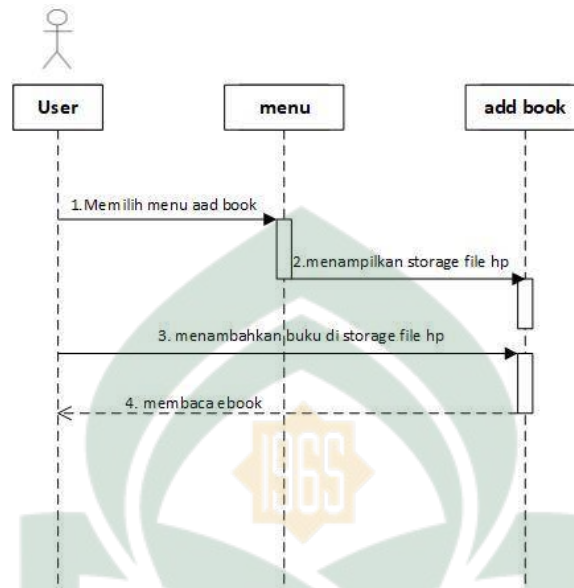
Gambar IV.7 Sequence Diagram Add Book
