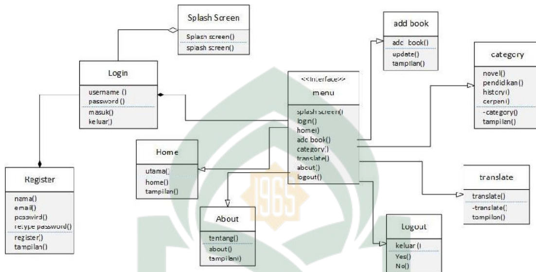
Gambar IV.4 Class Diagram
