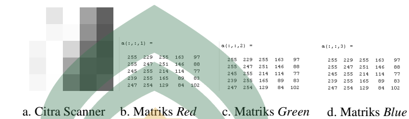
Gambar IV.6. Matriks Citra RGB Hasil Scanner
