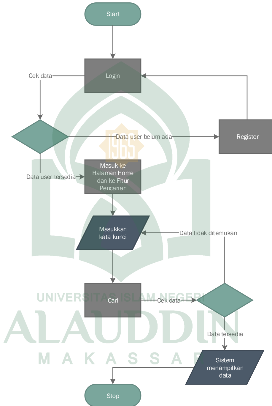
Gambar IV. 23 Flowchart Pencarian
